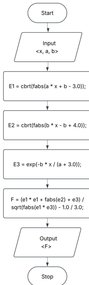
Fig. 4 - Block diagram of the program algorithm
