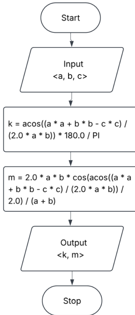
Fig. 2 – Block diagram of the program algorithm
