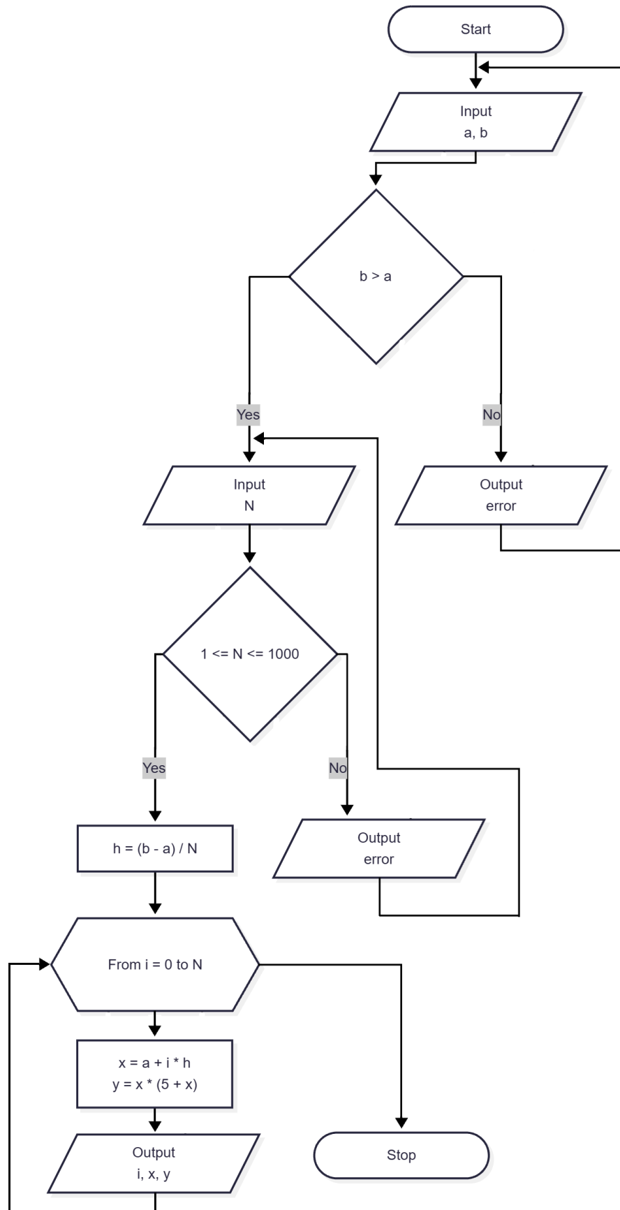
Fig. 1 – Block diagram of the program algorithm
