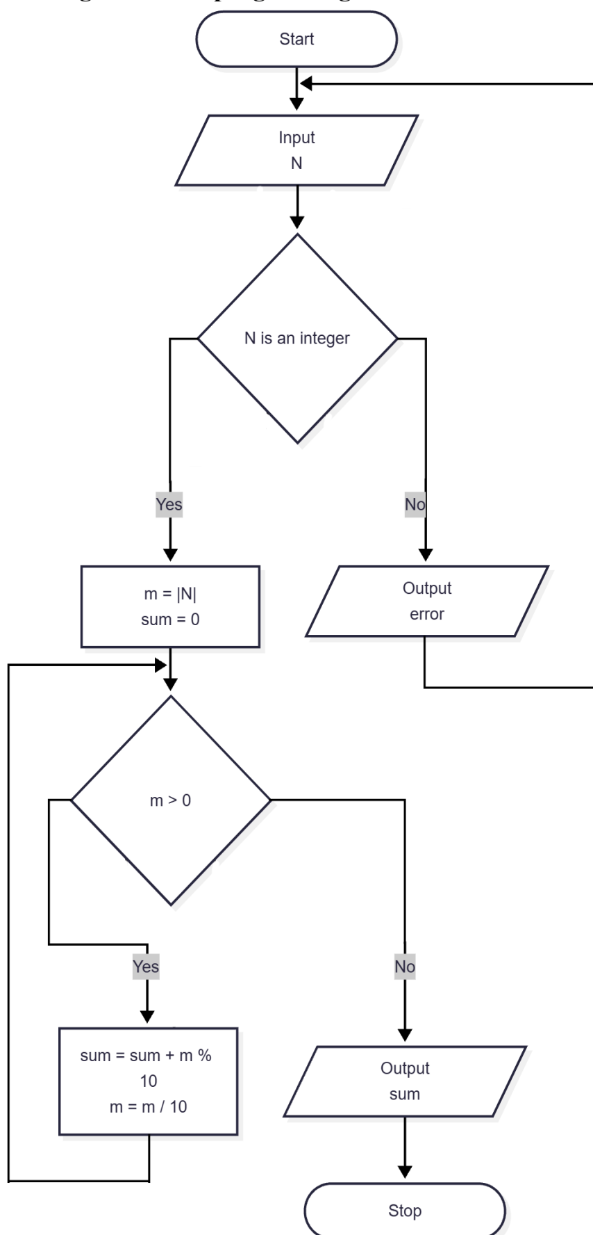
Fig. 5 – Block diagram of the program algorithm
