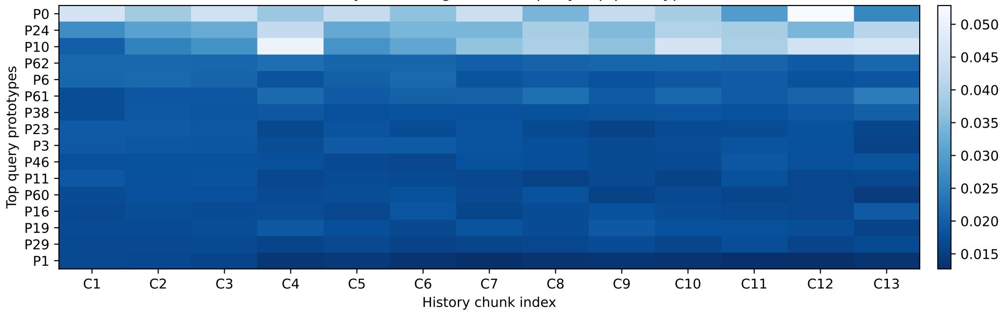
(c) Chunk weights
