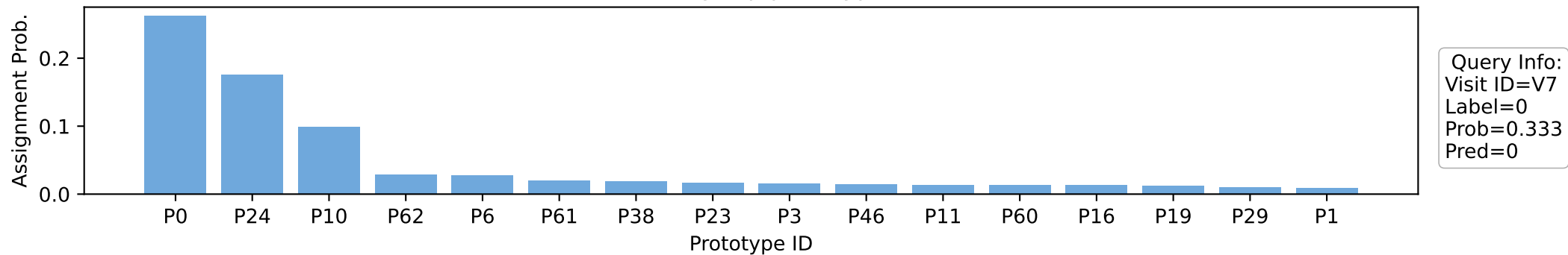
(b) History chunk alignment to query top prototypes
