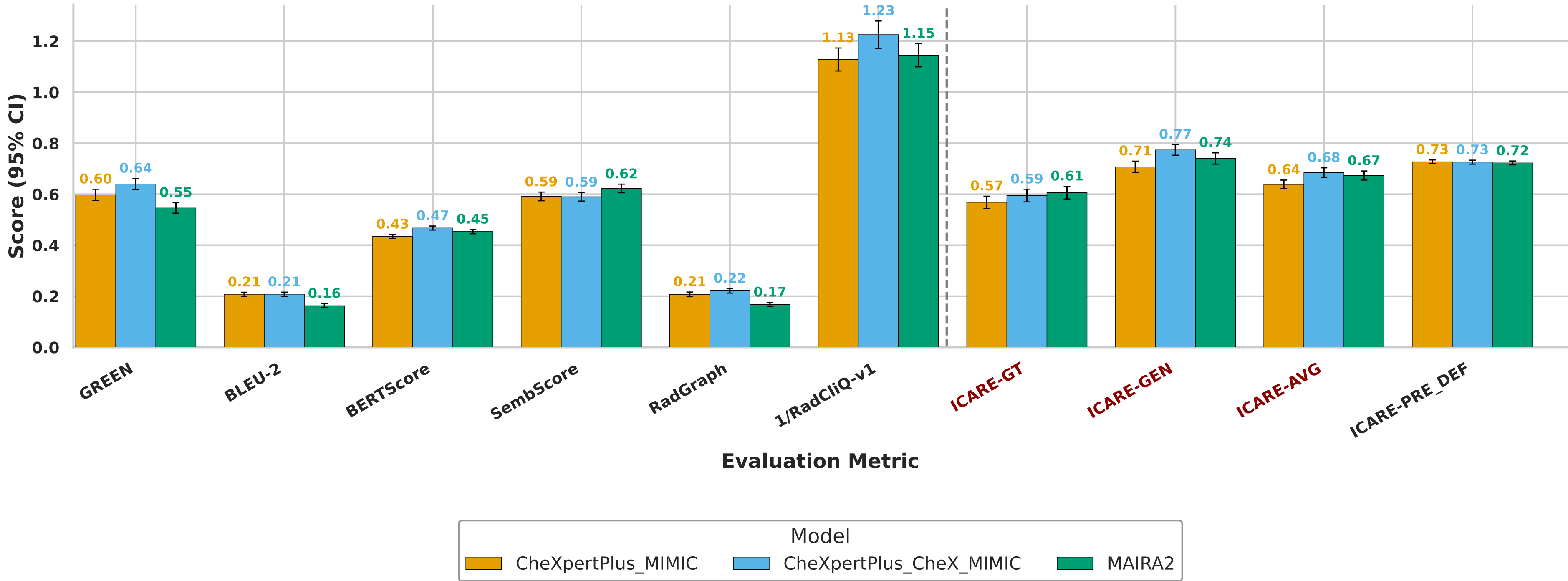
Quantitative Evaluation of RRG Models Across Metrics (IU Xray)
