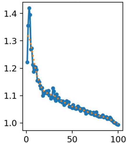
val/dfl_loss
