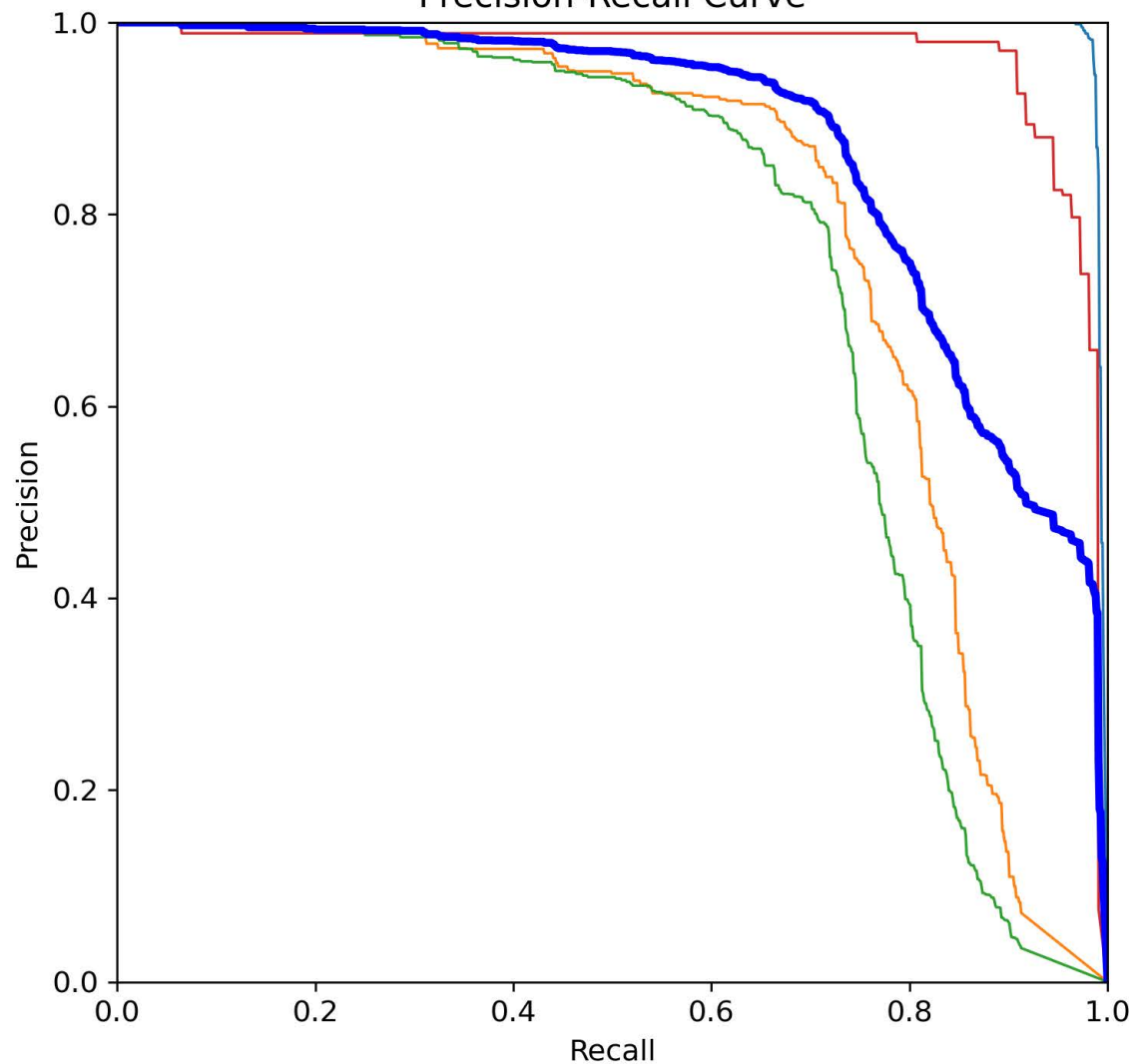
Precision-Recall Curve
