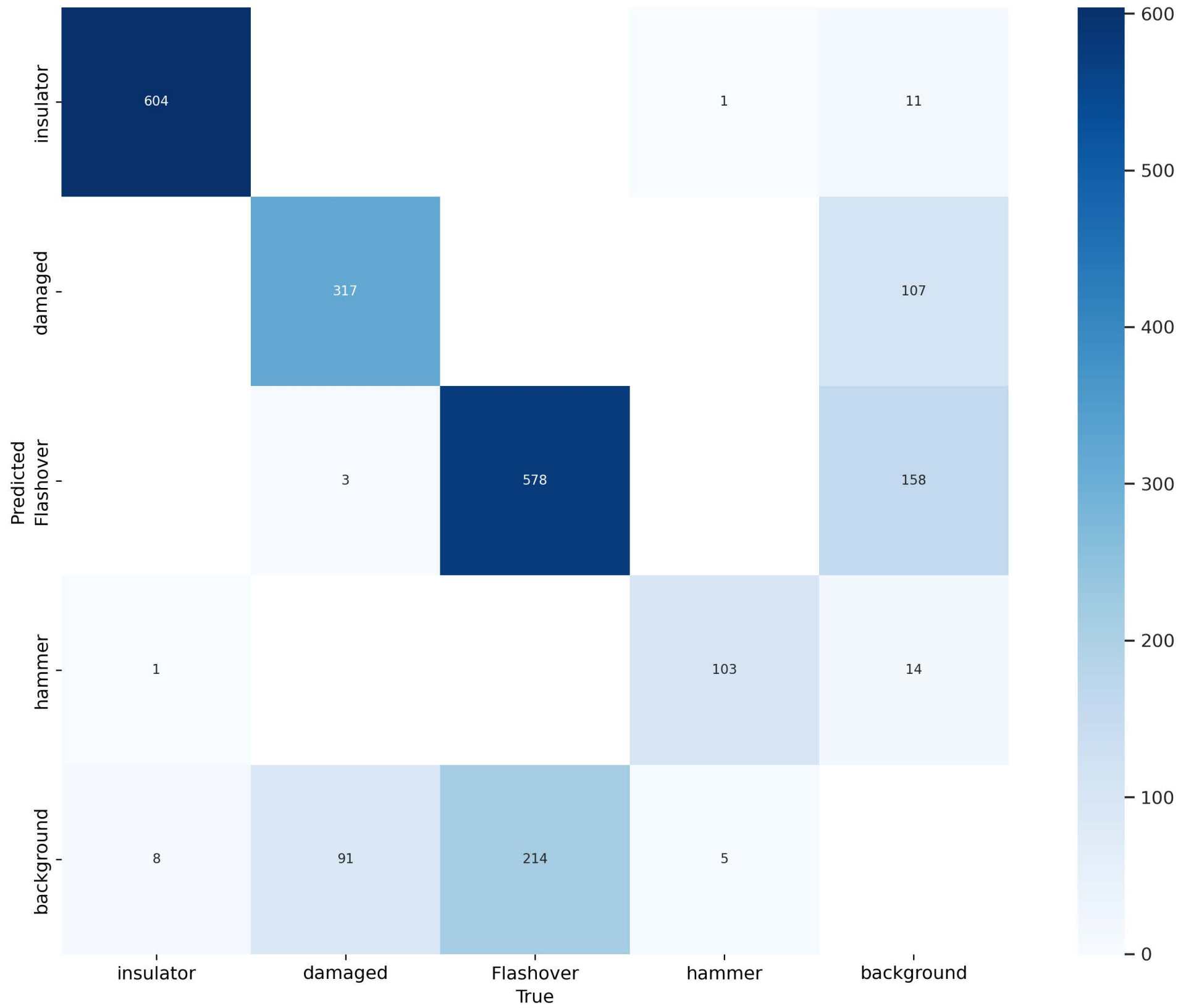
Confusion Matrix
