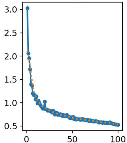
val/cls_loss
