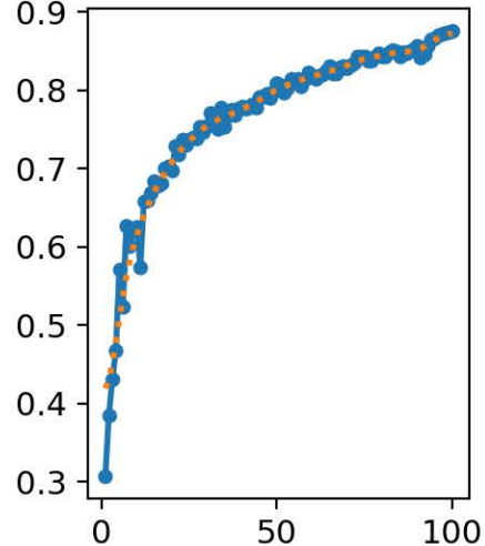
metrics/mAP50(B)
