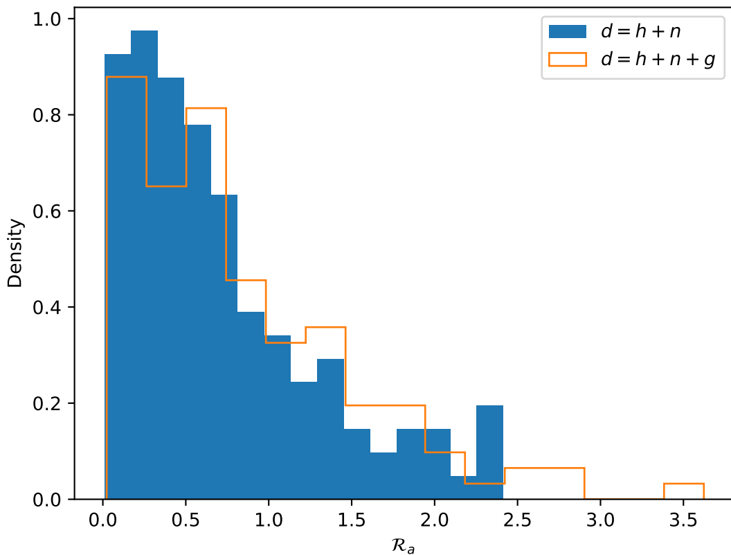
Estimates of \mathcal{R}_a for Prograde_EMRI over 128 glitch backgrounds
