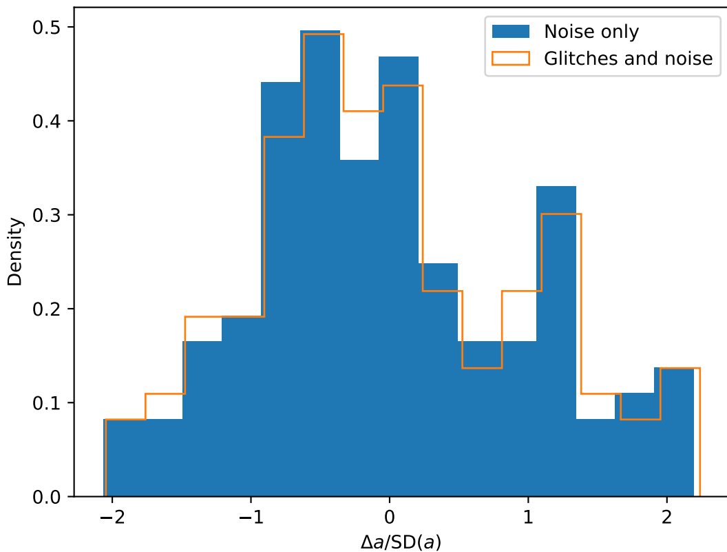
Estimated biases of a for Prograde_EMRI over 128 glitch backgrounds
