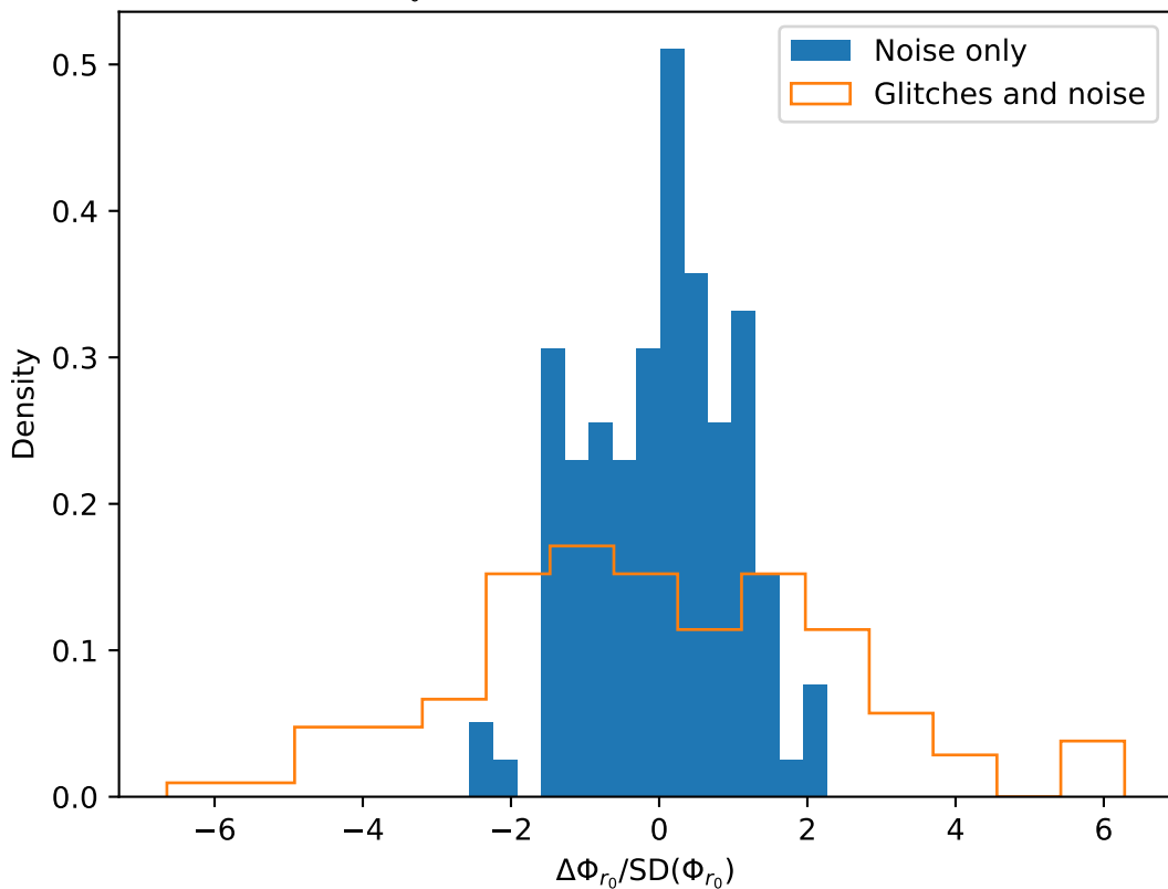
Estimated biases of \Phi_{r_0} for Prograde_EMRI over 122 glitch backgrounds
