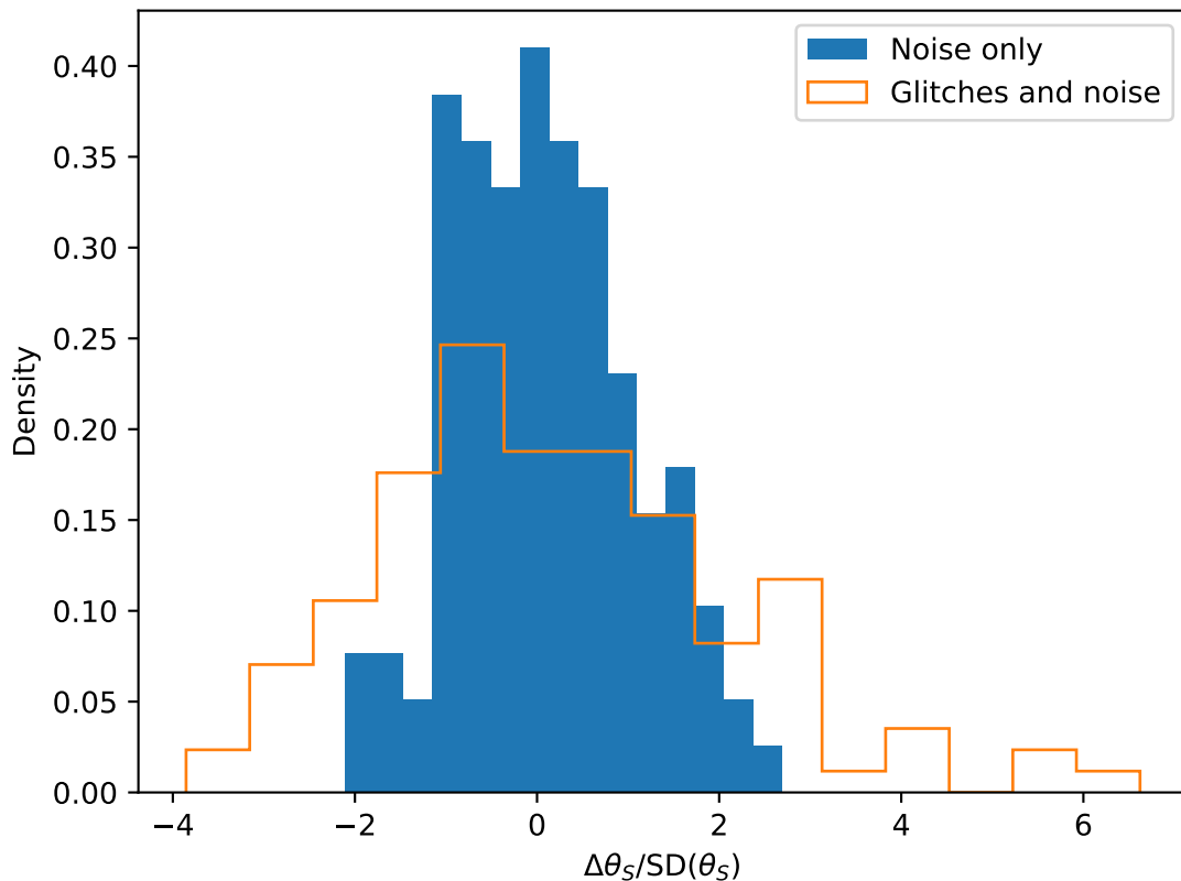
Estimated biases of \theta_S for Prograde_EMRI over 122 glitch backgrounds
