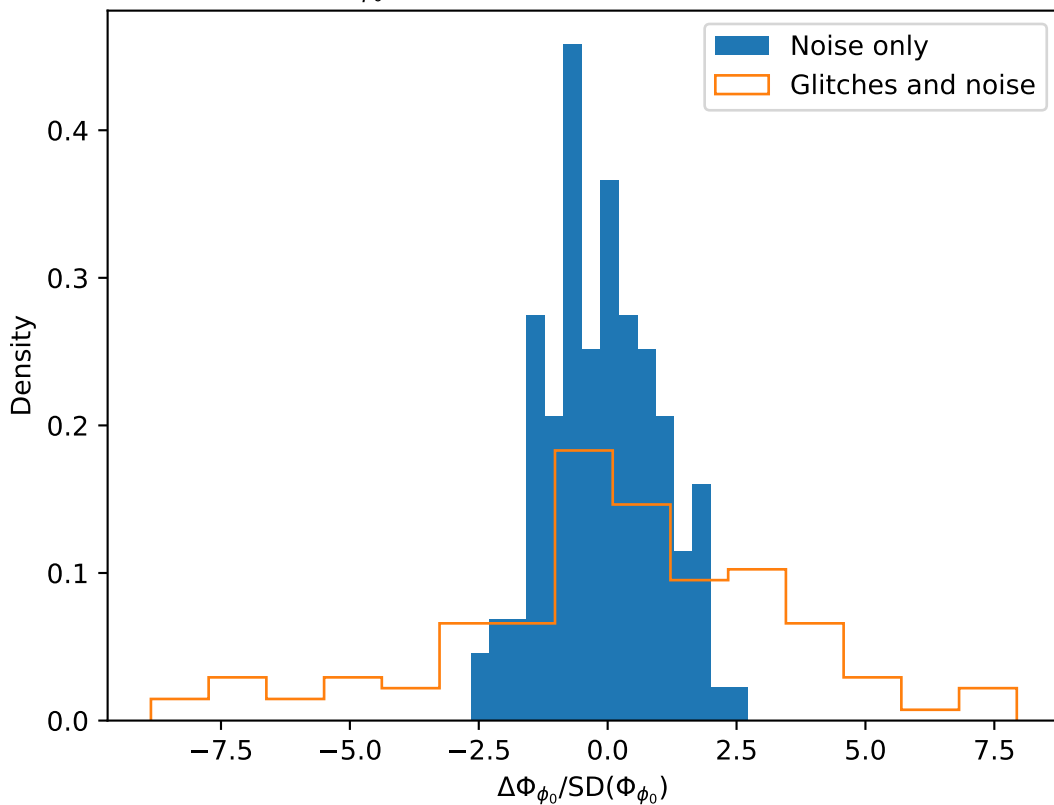
Estimated biases of \Phi_{\phi_0} for Prograde_EMRI over 122 glitch backgrounds
