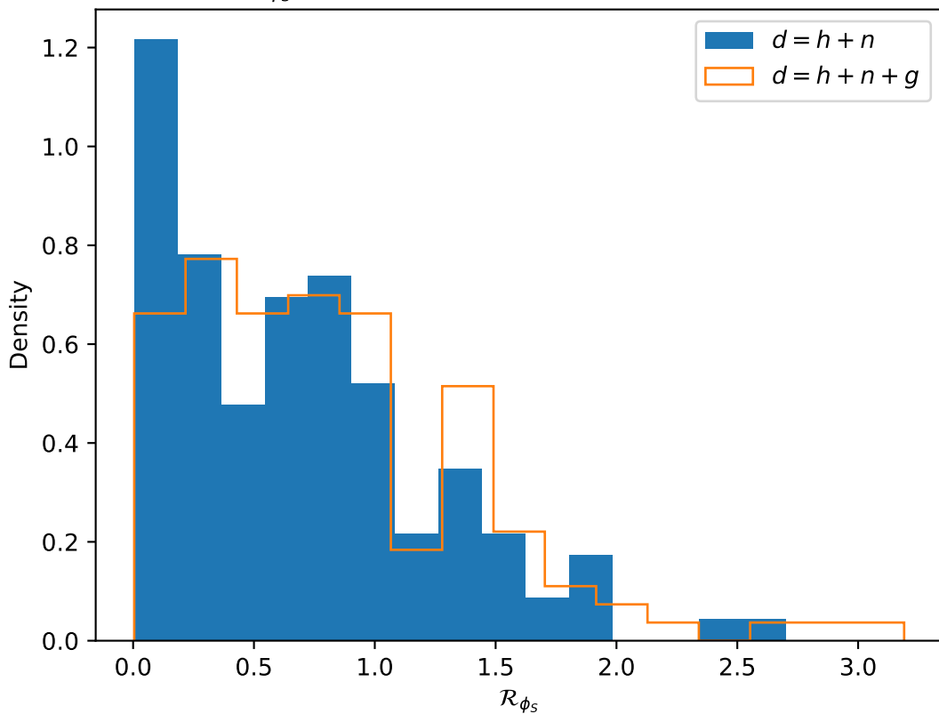
Estimates of \mathcal{R}_{\phi_s} for Prograde_EMRI over 128 glitch backgrounds
