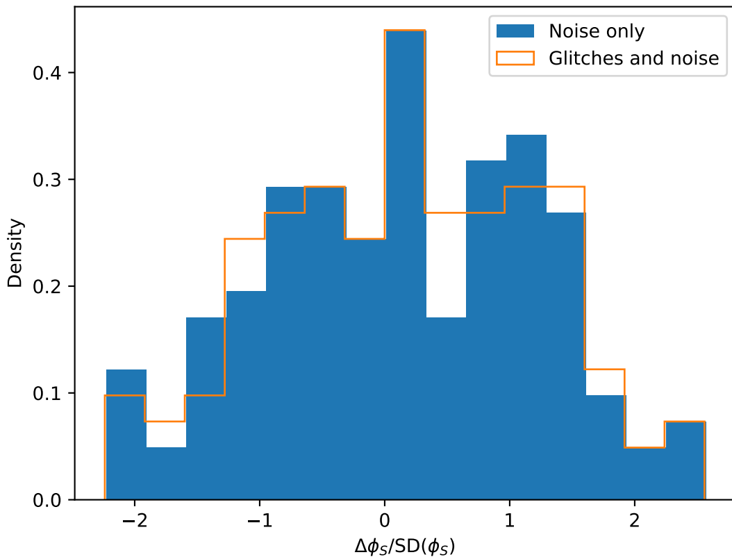
Estimated biases of \phi_S for Prograde_EMRI over 128 glitch backgrounds
