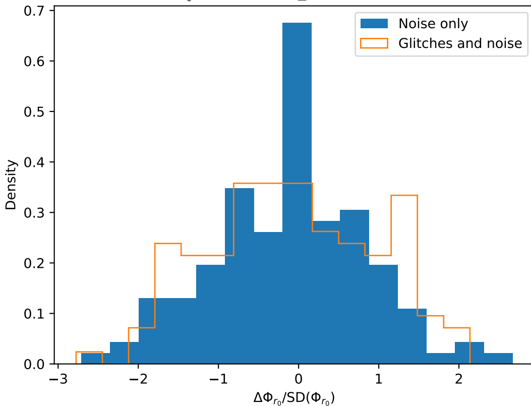
Estimated biases of \Phi_{r_0} for Prograde_EMRI over 128 glitch backgrounds
