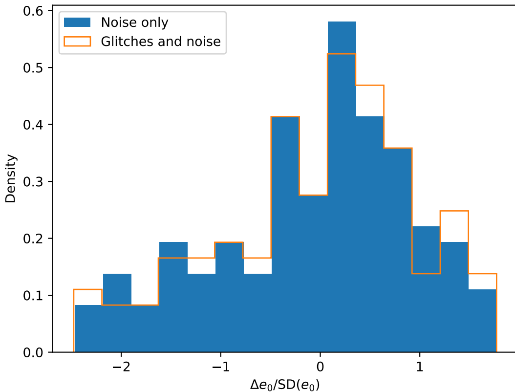
Estimated biases of e_0 for Prograde_EMRI over 128 glitch backgrounds
