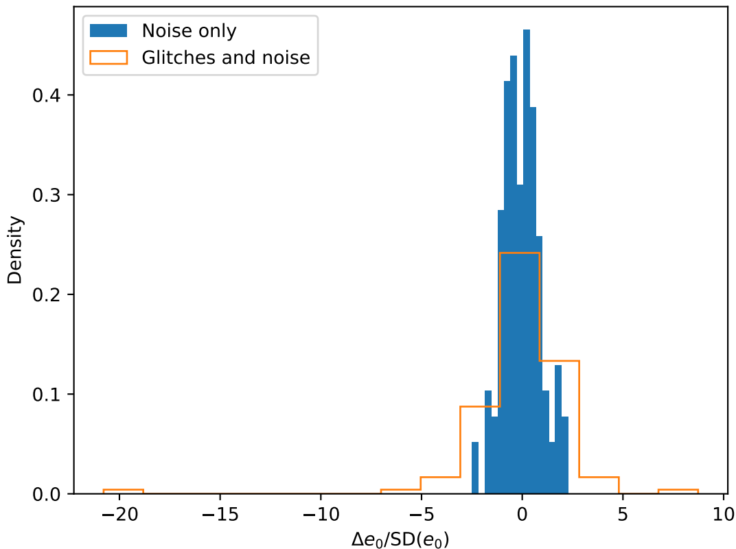
Estimated biases of e_0 for Prograde_EMRI over 122 glitch backgrounds
