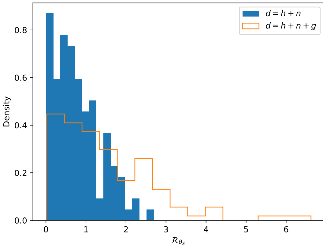
Estimates of \mathcal{R}_{\theta_s} for Prograde_EMRI over 122 glitch backgrounds
