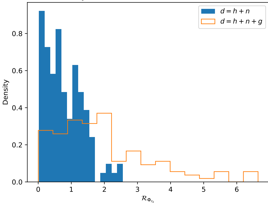
Estimates of \mathcal{R}_{\Phi_{r_0}} for Prograde_EMRI over 122 glitch backgrounds
