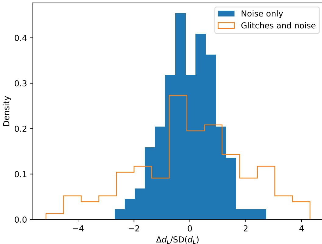
Estimated biases of d_L for Prograde_EMRI over 122 glitch backgrounds
