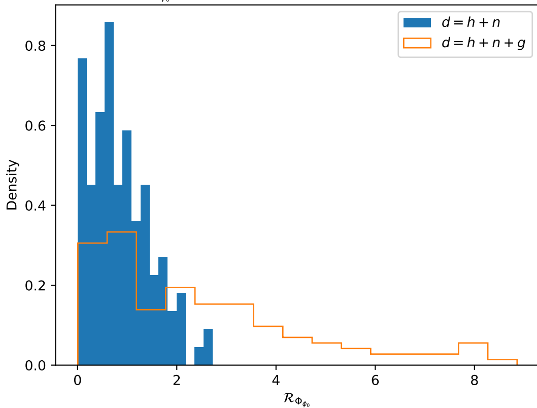
Estimates of \mathcal{R}_{\Phi_{\phi_0}} for Prograde_EMRI over 122 glitch backgrounds
