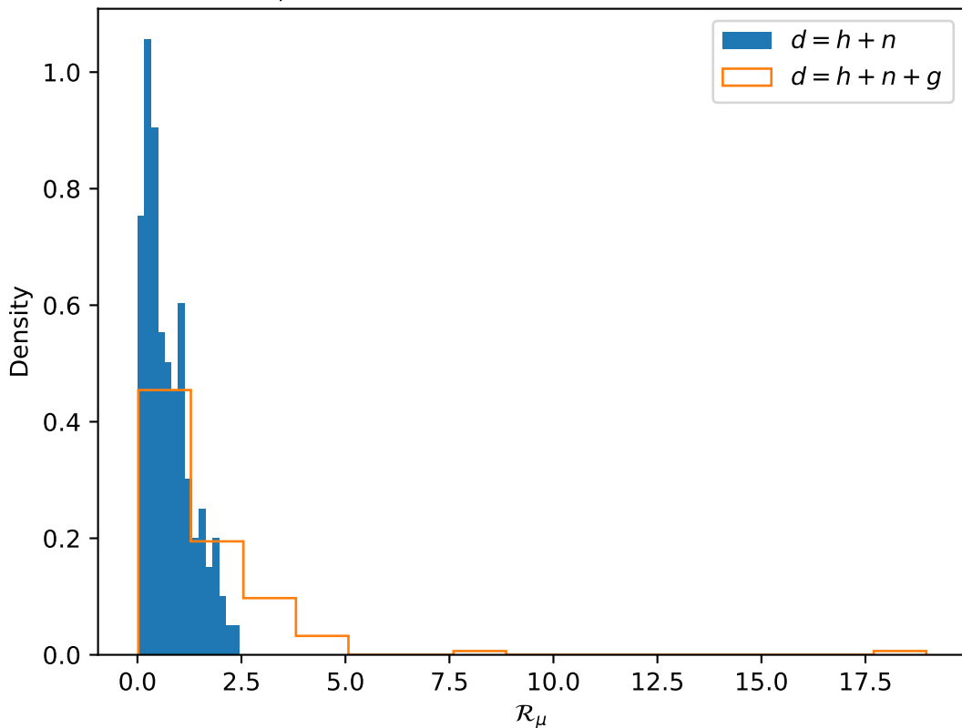
Estimates of \mathcal{R}_\mu for Prograde_EMRI over 122 glitch backgrounds
