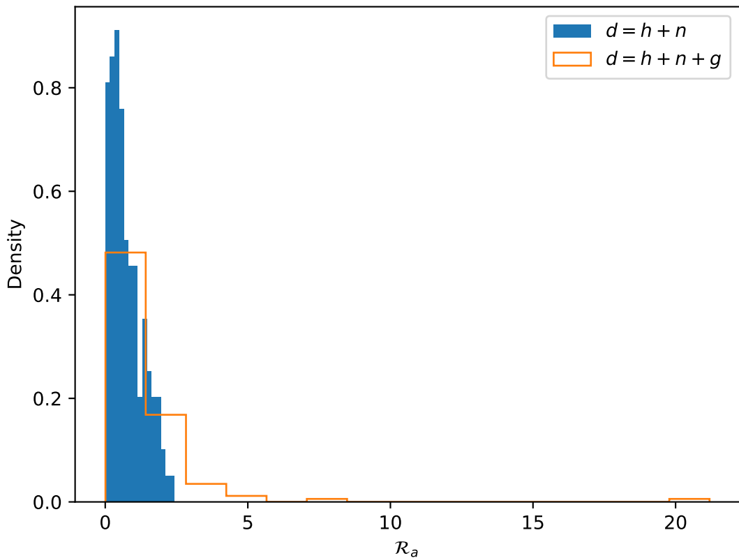
Estimates of \mathcal{R}_a for Prograde_EMRI over 122 glitch backgrounds
