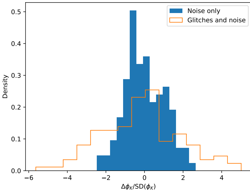
Estimated biases of \phi_K for Prograde_EMRI over 122 glitch backgrounds
