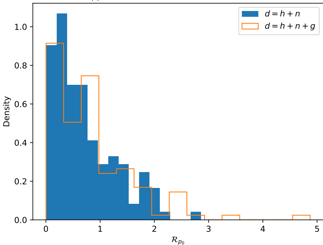
Estimates of \mathcal{R}_{p_0} for Prograde_EMRI over 128 glitch backgrounds
