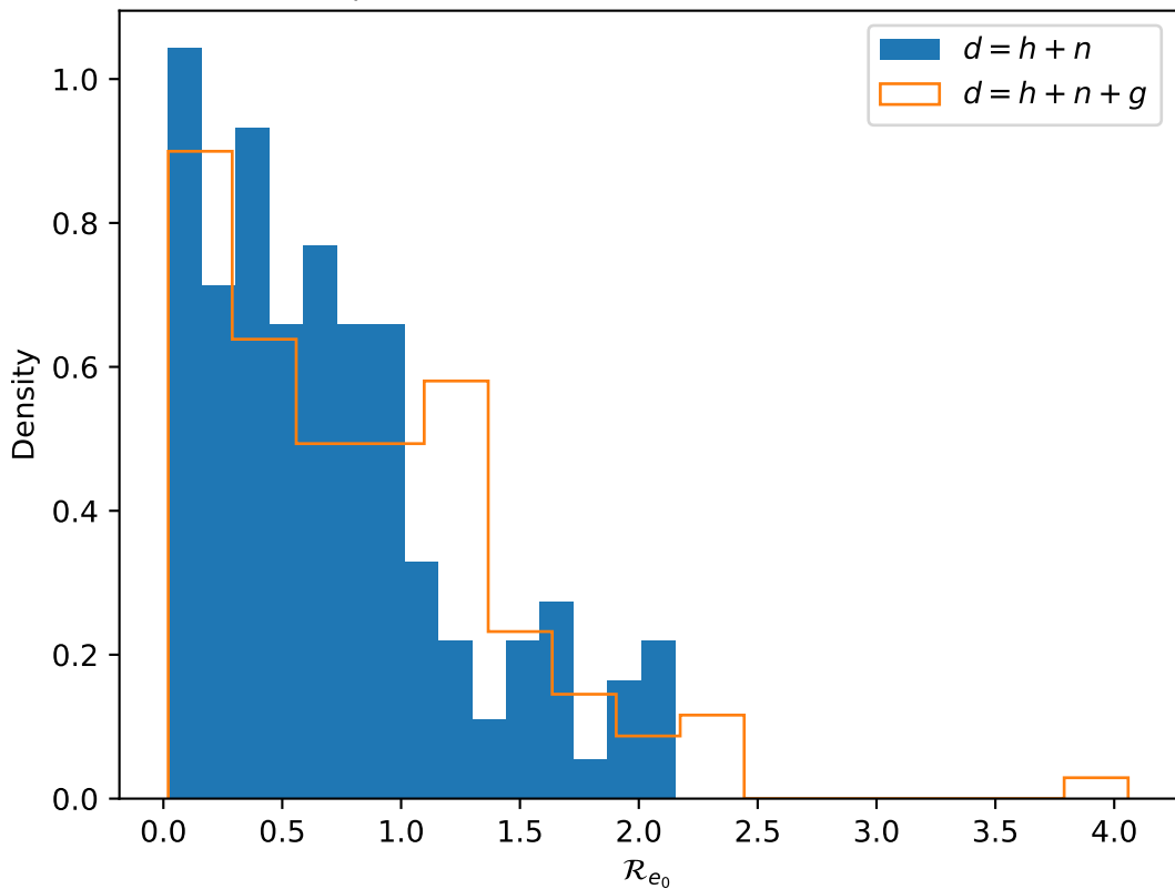
Estimates of \mathcal{R}_{e_0} for Prograde_EMRI over 128 glitch backgrounds
