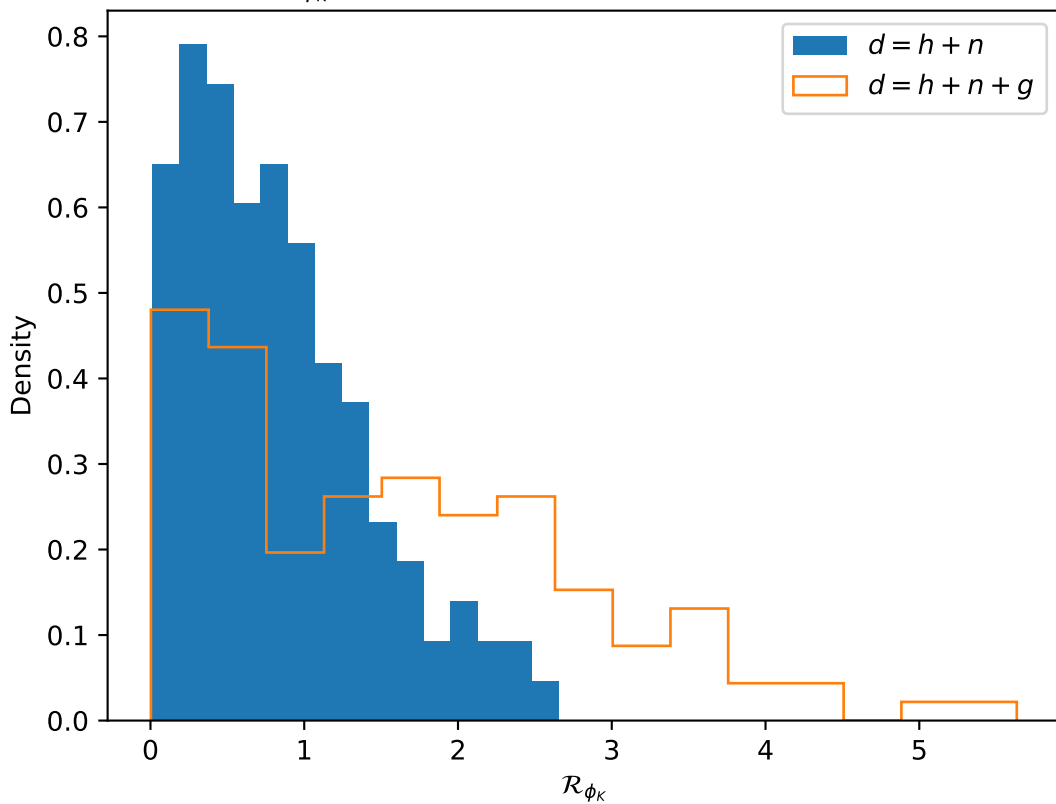
Estimates of \mathcal{R}_{\phi_K} for Prograde_EMRI over 122 glitch backgrounds
