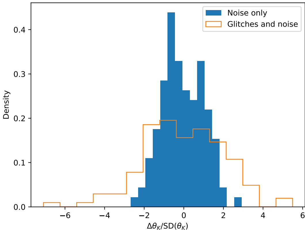
Estimated biases of \theta_K for Prograde_EMRI over 122 glitch backgrounds
