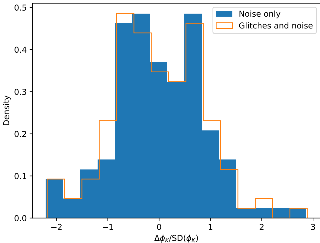
Estimated biases of \phi_K for Prograde_EMRI over 128 glitch backgrounds
