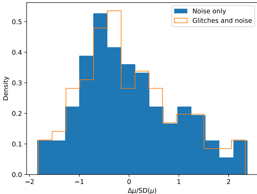
Estimated biases of \mu for Prograde_EMRI over 128 glitch backgrounds
