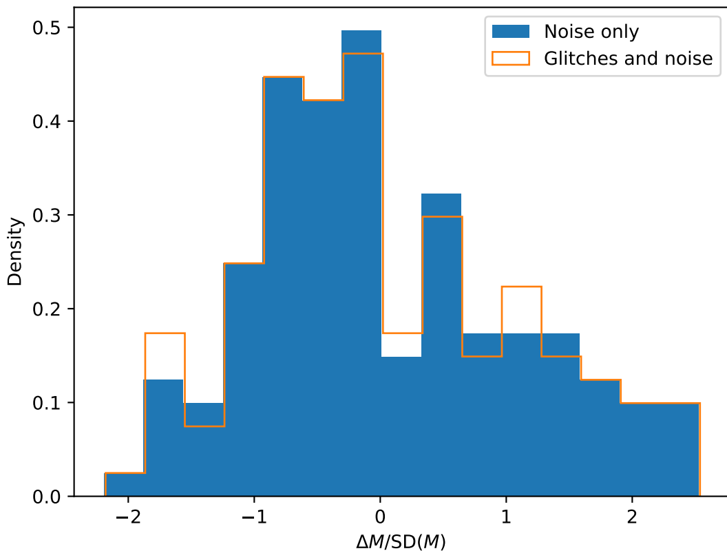
Estimated biases of M for Prograde_EMRI over 128 glitch backgrounds
