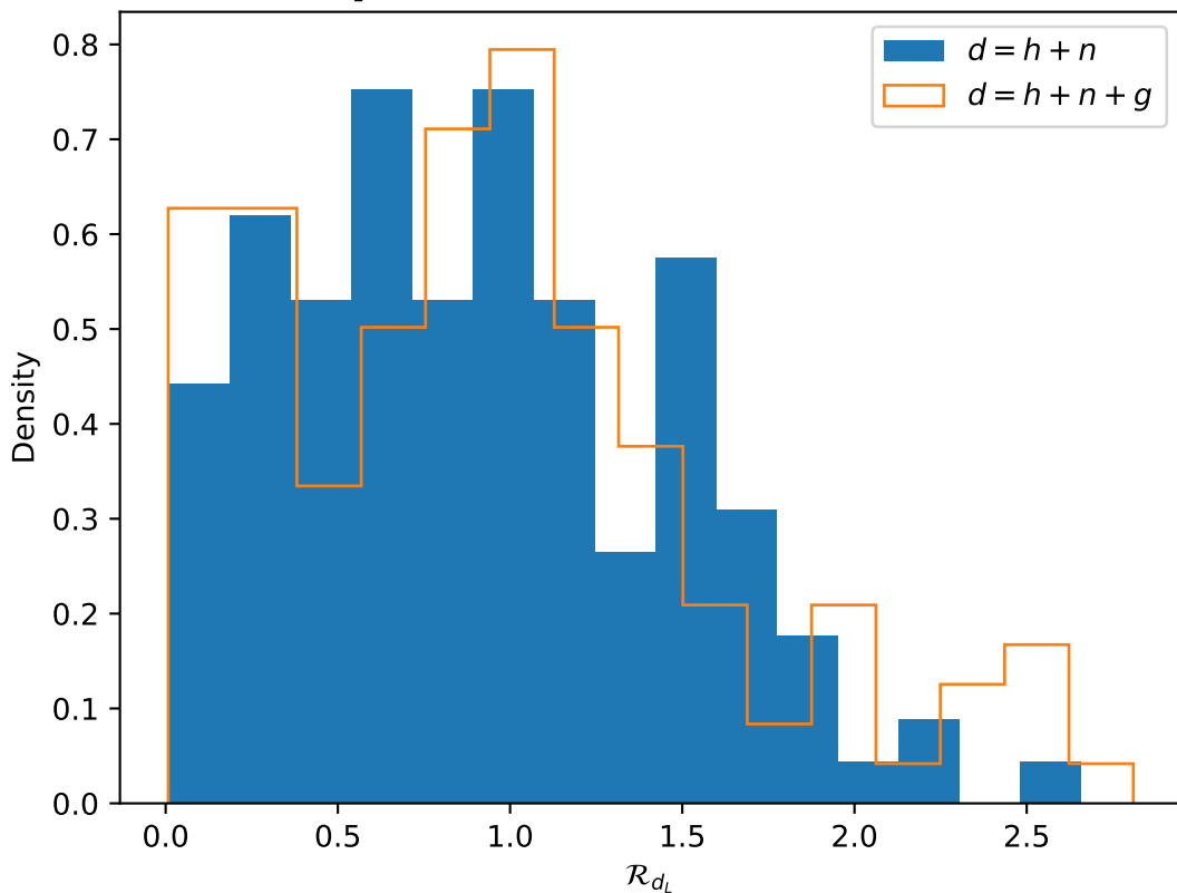
Estimates of \mathcal{R}_{d_L} for Prograde_EMRI over 128 glitch backgrounds
