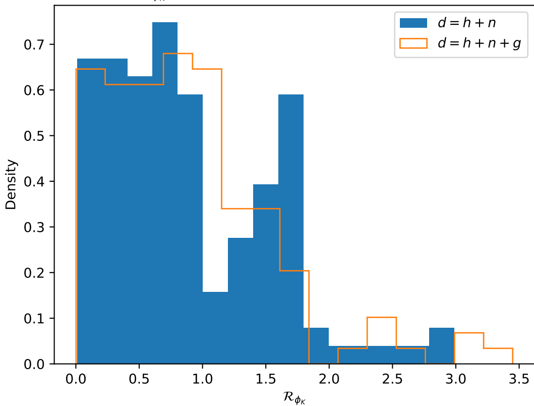
Estimates of \mathcal{R}_{\phi_K} for Prograde_EMRI over 128 glitch backgrounds
