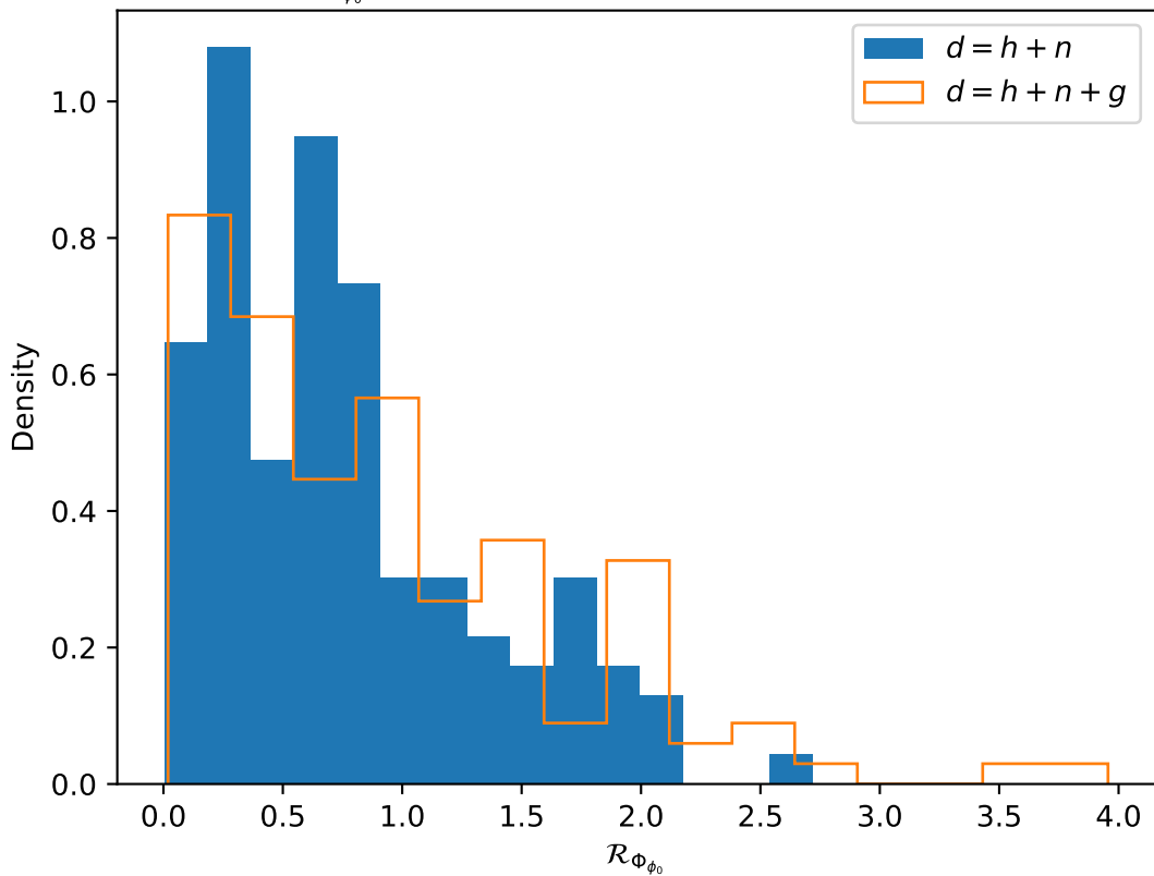
Estimates of \mathcal{R}_{\Phi_{\phi_0}} for Prograde_EMRI over 128 glitch backgrounds
