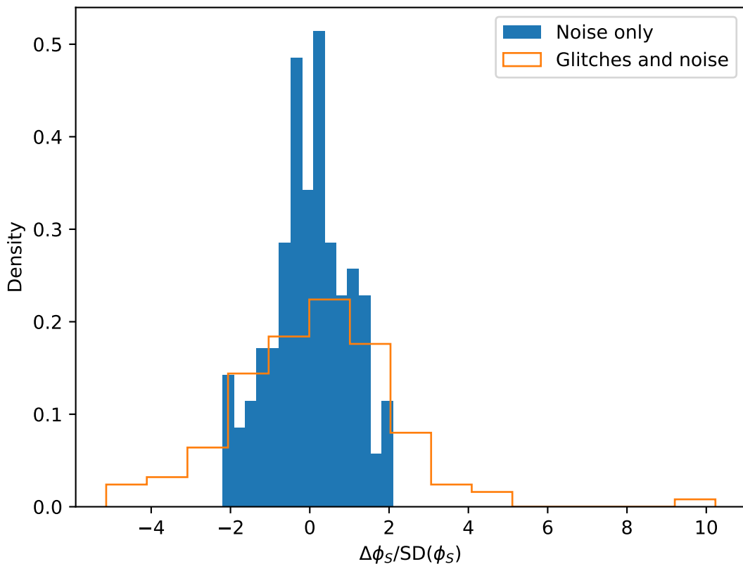
Estimated biases of \phi_S for Prograde_EMRI over 122 glitch backgrounds
