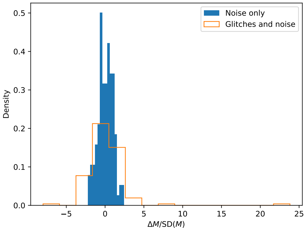
Estimated biases of M for Prograde_EMRI over 122 glitch backgrounds
