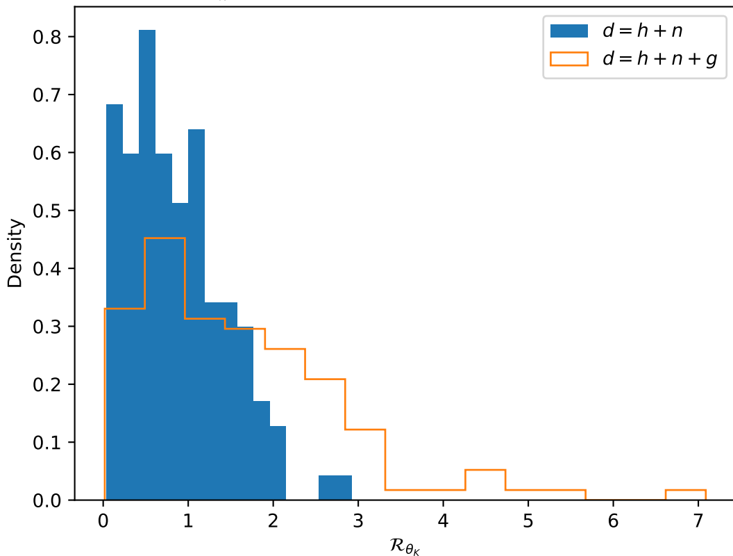
Estimates of \mathcal{R}_{\theta_k} for Prograde_EMRI over 122 glitch backgrounds
