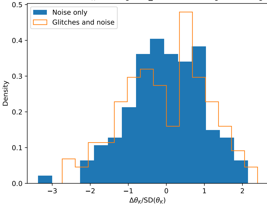
Estimated biases of \theta_K for Prograde_EMRI over 128 glitch backgrounds
