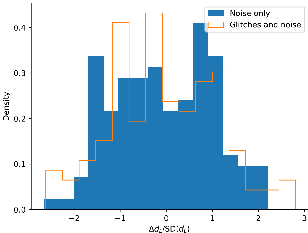
Estimated biases of d_L for Prograde_EMRI over 128 glitch backgrounds
