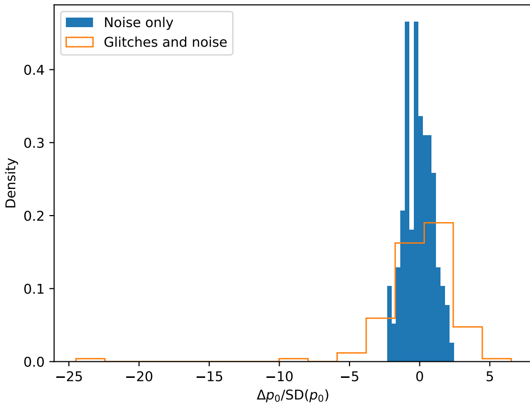
Estimated biases of p_0 for Prograde_EMRI over 122 glitch backgrounds
