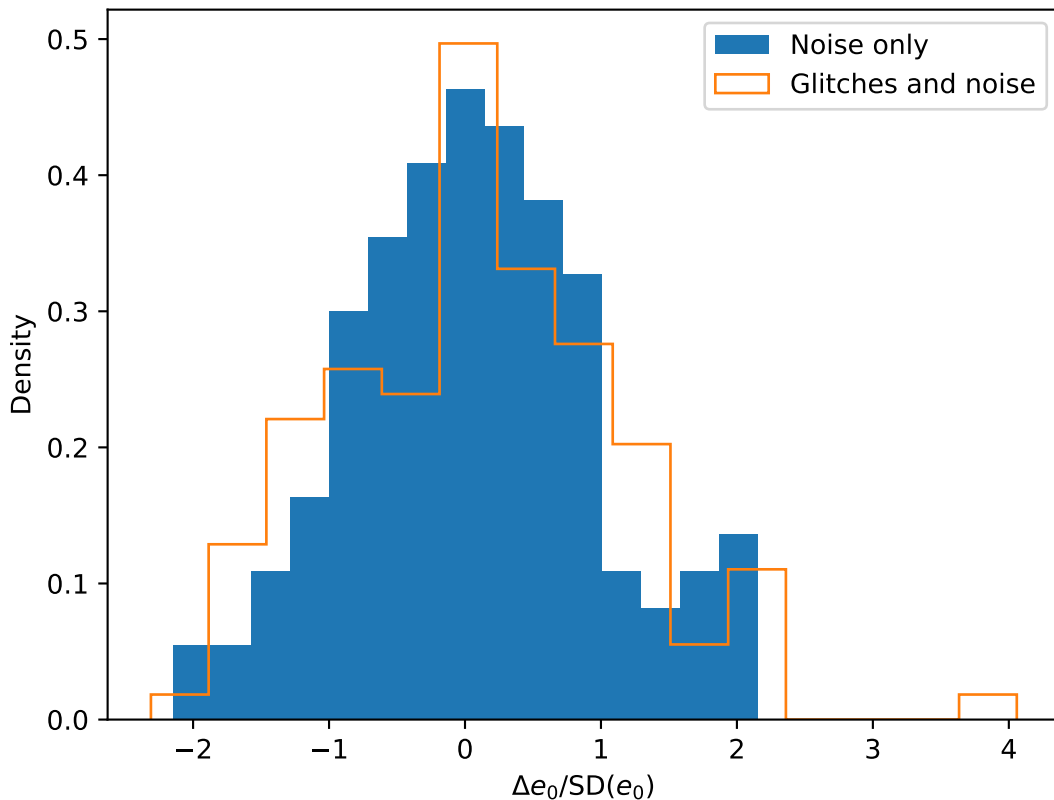
Estimated biases of e_0 for Prograde_EMRI over 128 glitch backgrounds
