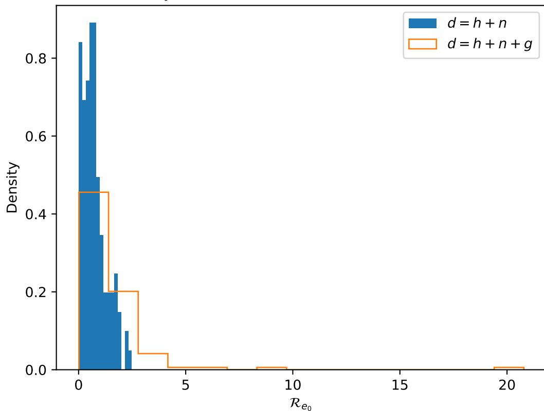
Estimates of \mathcal{R}_{e_0} for Prograde_EMRI over 122 glitch backgrounds
