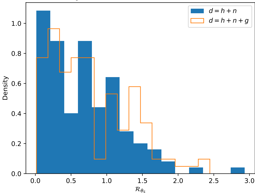
Estimates of \mathcal{R}_{\theta_s} for Prograde_EMRI over 128 glitch backgrounds
