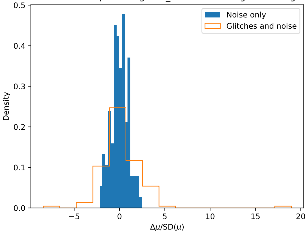
Estimated biases of \mu for Prograde_EMRI over 122 glitch backgrounds
