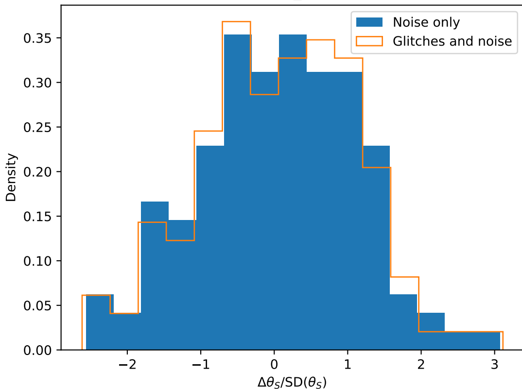
Estimated biases of \theta_S for Prograde_EMRI over 128 glitch backgrounds
