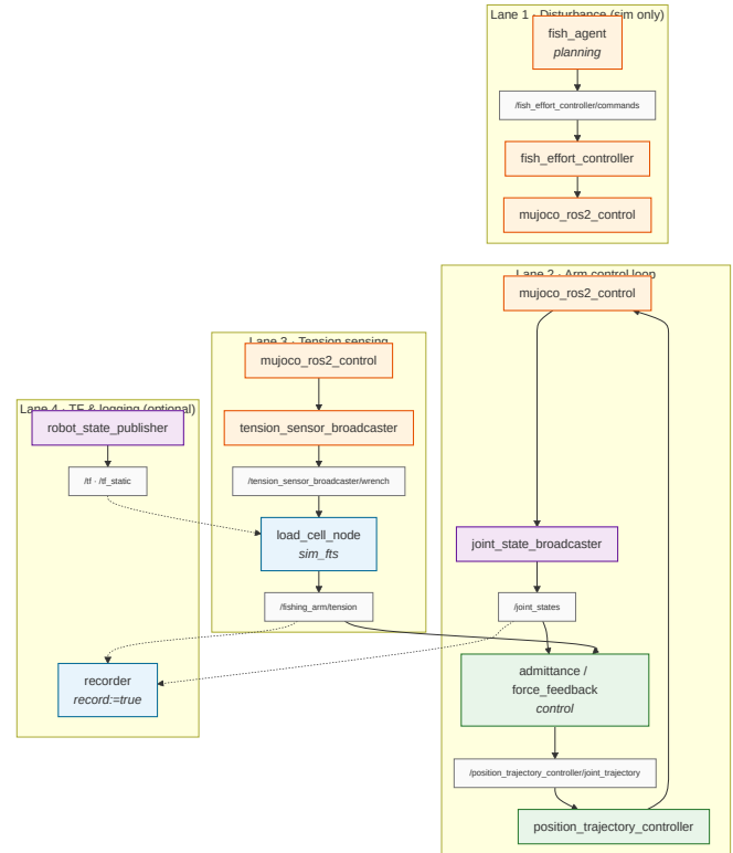
Fig. 7: Software ROS2 graph
