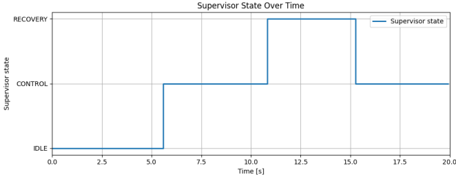
Fig. 14: Engagement and recovery supervisor state during the hardware trial.
