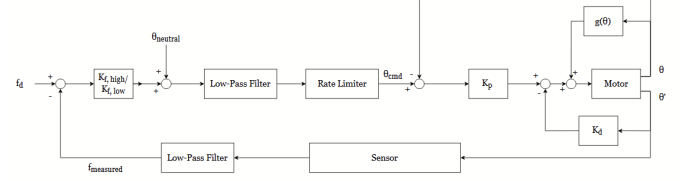
Fig. 10: Proportional Force Control diagram.
