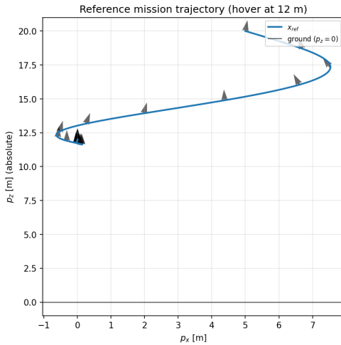
Fig. 11: Reference mission trajectory in the p_x - p_z plane with attitude.
