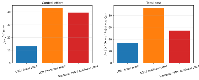
Fig. 28: Control effort J_u = \int u^T R u dt and total cost J .
