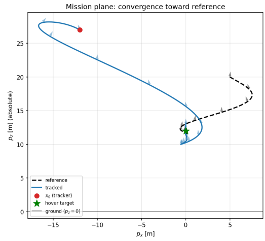
Fig. 12: Closed-loop convergence of the tracker onto the reference, with attitude arrows and the ground constraint p_z = 0 .
