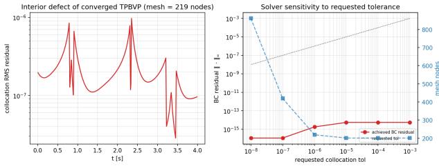
Fig. 30: Collocation convergence and tolerance sensitivity.
