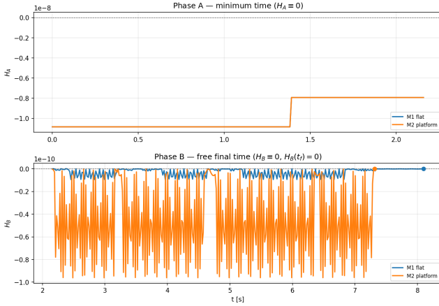
Fig. 24: Hamiltonian consistency: H_A \equiv 0 on Phase A (minimum time) and H_B \equiv 0 on Phase B (free final time), both to numerical tolerance.
