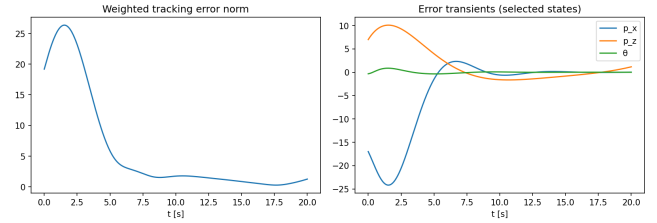
Fig. 13: Transient Response
