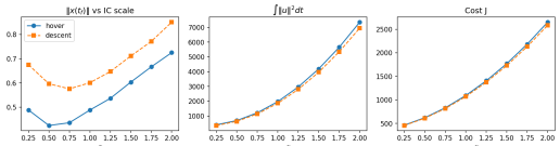
Fig. 3: Sensitivity to initial condition error
