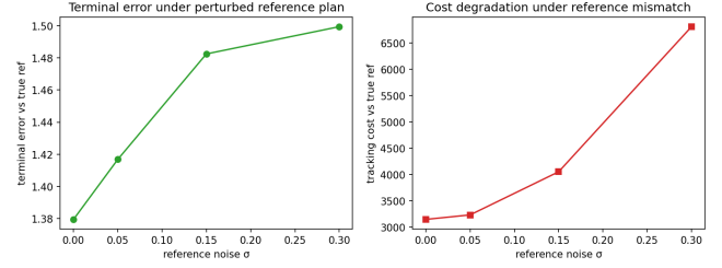
Fig. 17: Sensitivity to a perturbed reference plan: terminal error and cost (scored against the true reference) versus reference noise level \sigma .
