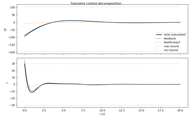
Fig. 14: Transient Control Decomposition
