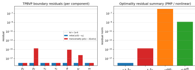
Fig. 32: Per-component TPBVP boundary and optimality residuals.
