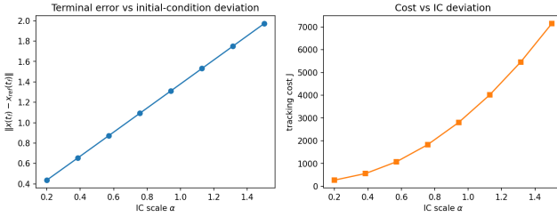
Fig. 16: Robustness to initial-condition deviations: terminal error and tracking cost as the initial offset is scaled by \alpha .
