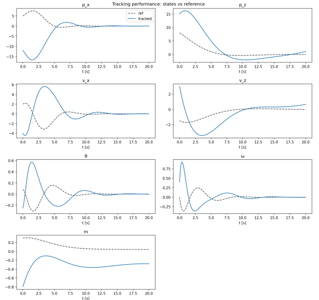
Fig. 9: Tracking Performance
