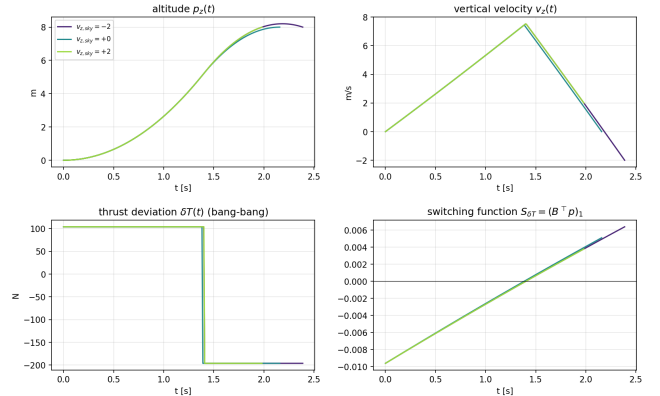
Fig. 19: Phase A minimum-time ascent for terminal vertical velocities
