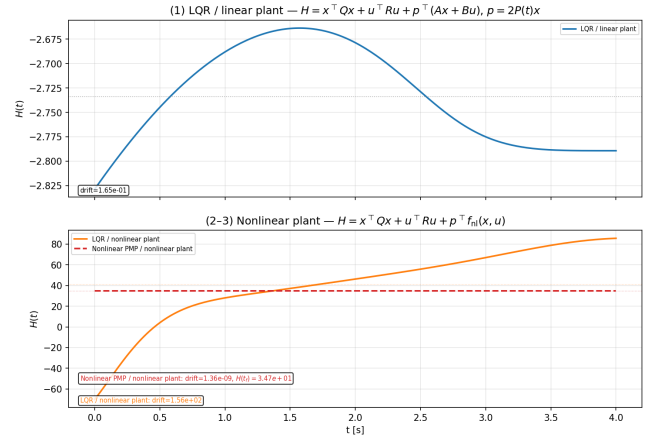
Fig. 33: Hamiltonian evolution H(t) for the three scenarios. The nonlinear PMP solution (bottom) holds H constant to \mathcal{O}(10^{-9}) as required for an autonomous fixed-time extremal, whereas the LQR law on the nonlinear plant drifts by \mathcal{O}(10^2) .
