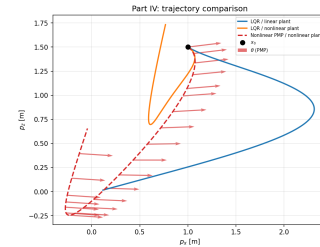
Fig. 26: Mission plane p_x vs. p_z with attitude vectors.
