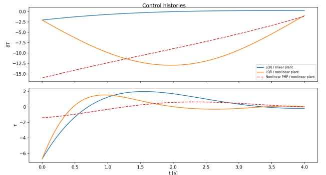
Fig. 27: Thrust and torque histories.
