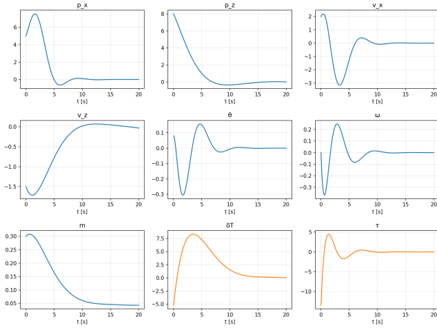
Fig. 10: Recorded Part I optimal trajectory used as the reference x_{\text{ref}}(t) , u_{\text{ref}}(t) .
