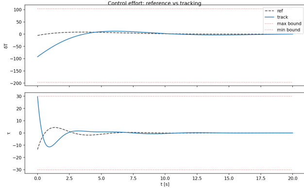
Fig. 15: Control Effort
