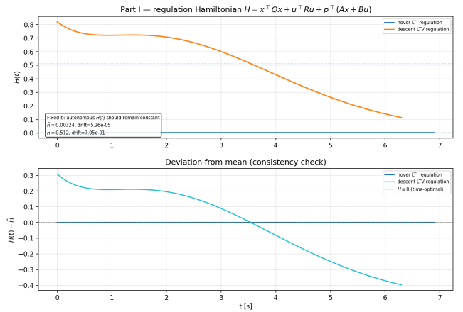
Fig. 8: Hamiltonian evolution
