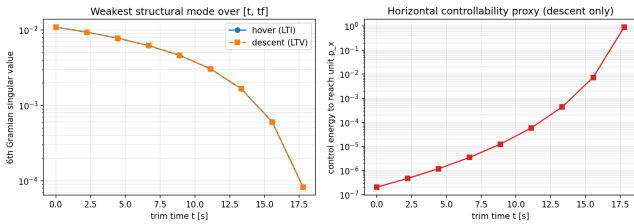
Fig. 2: Controllability Gramian and horizontal controllability proxy
