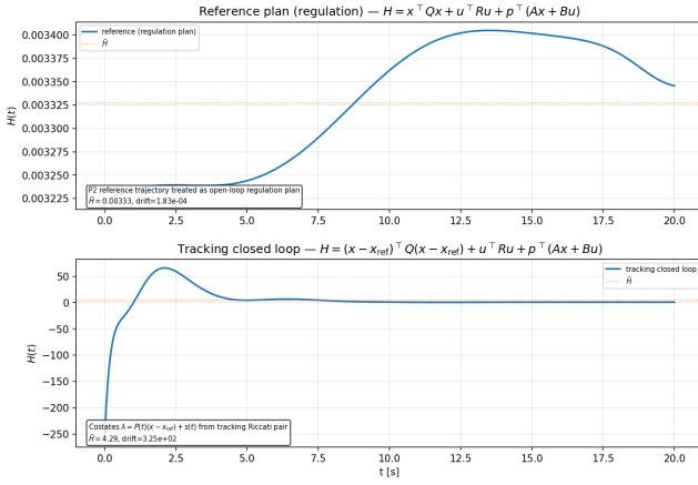
Fig. 18: Hamiltonian consistency: constant for the autonomous reference plan and time-varying for the tracking problem.
