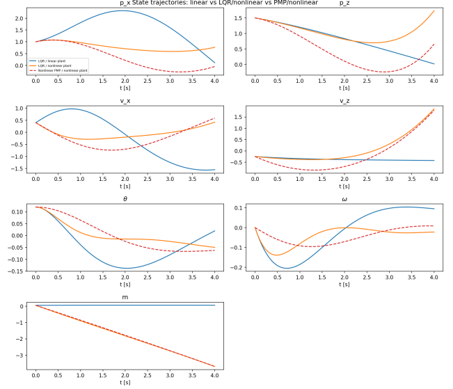
Fig. 25: State trajectories for the three scenarios.
