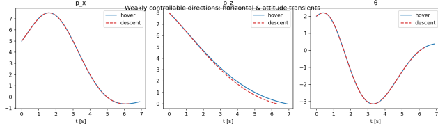
Fig. 5: Transient behavior
