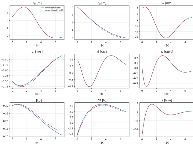
Fig. 6: Optimal solution trajectories versus time: states and control histories.
