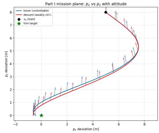
Fig. 7: Mission-plane trajectory ( p_x vs p_z ) with attitude vectors at sampled positions.
