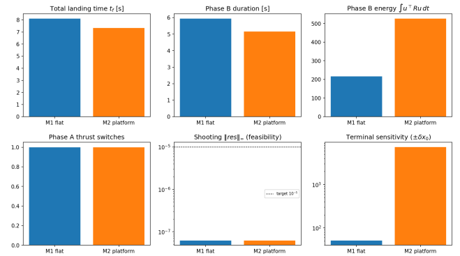
Fig. 23: M1 vs M2 comparison: total landing time t_f , Phase B duration, Phase B control energy \int u^\top R u dt , Phase A thrust switches, shooting feasibility \|res\|_\infty , and terminal sensitivity to \pm 0.05 handoff perturbations.
