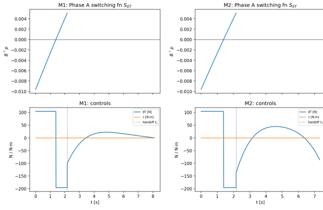
Fig. 20: Phase A switching function S_{\delta T}(t) (top) and full mission control histories \delta T(t) , \tau(t) (bottom) for M1 and M2; the dotted line marks the Phase A/Phase B handoff t_1 . The single sign change of S_{\delta T} confirms the bang–bang structure with one switch.
