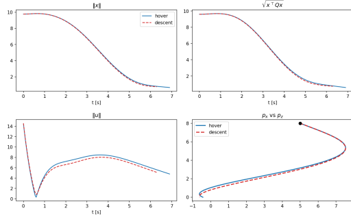
Fig. 4: State and control effort across trajectory
