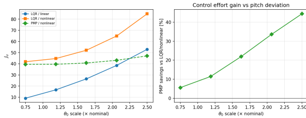
Fig. 31: Control effort and PMP savings vs. scaled initial pitch \theta_0 .
