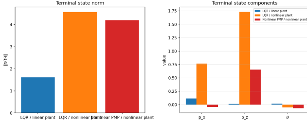
Fig. 29: Terminal state norm and components at t_f .
