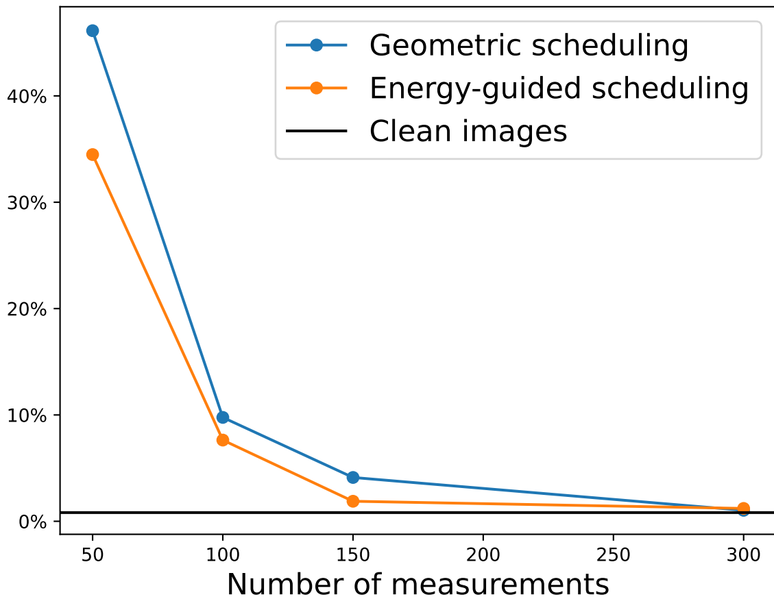
Classification error
