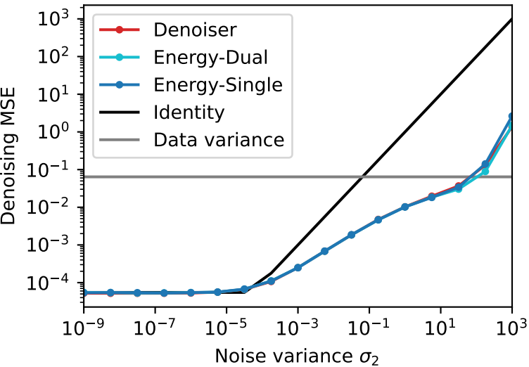
Box inpainting ( \sigma_1 = 10^{-3} )
