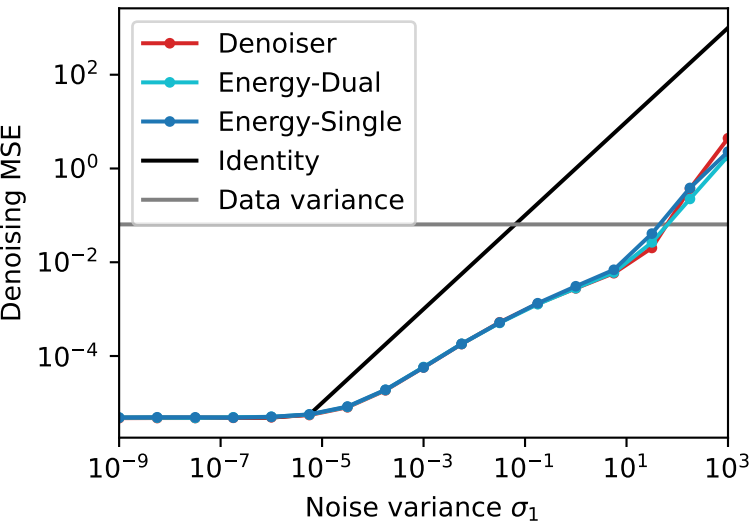
Box inpainting ( \sigma_2 = 10^{-5} )
