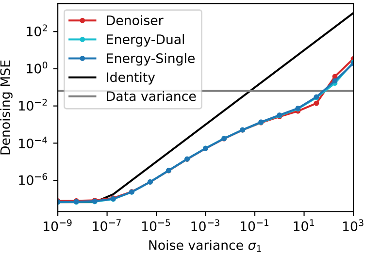
Box inpainting ( \sigma_2 = 10^{-7} )
