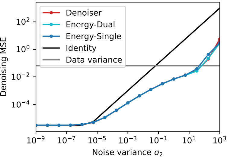
Box inpainting ( \sigma_1 = 10^{-5} )
