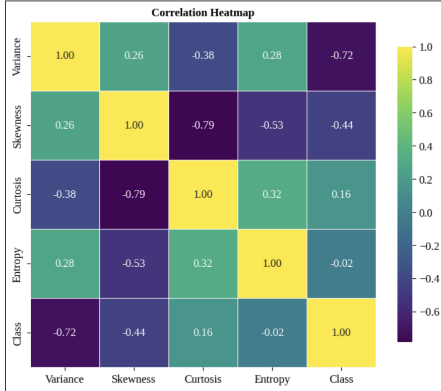
Figure 6: Correlation Heatmap.
