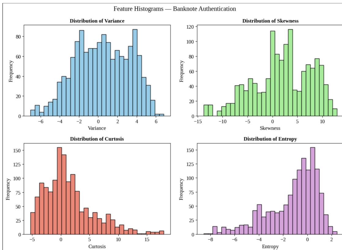
Figure 5: Feature Histograms.
