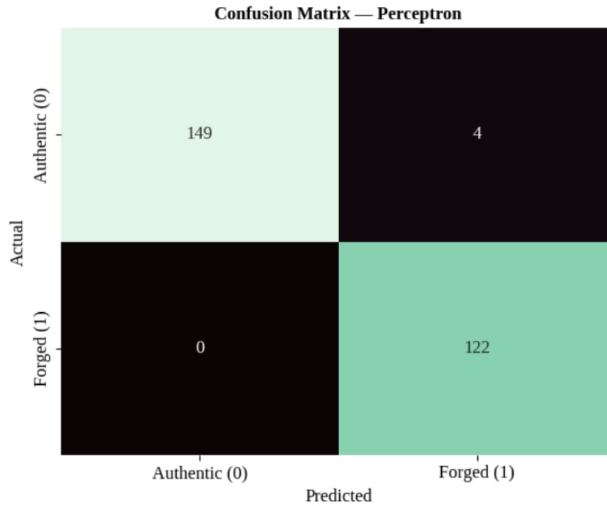
Figure 12: Confusion Matrix.
