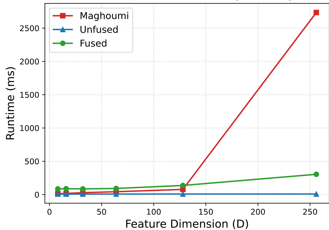
Runtime vs. Dimension (L = 256)
