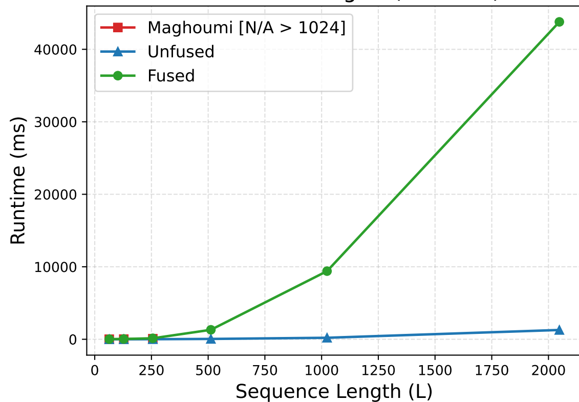
Runtime vs. Length (D = 128)
