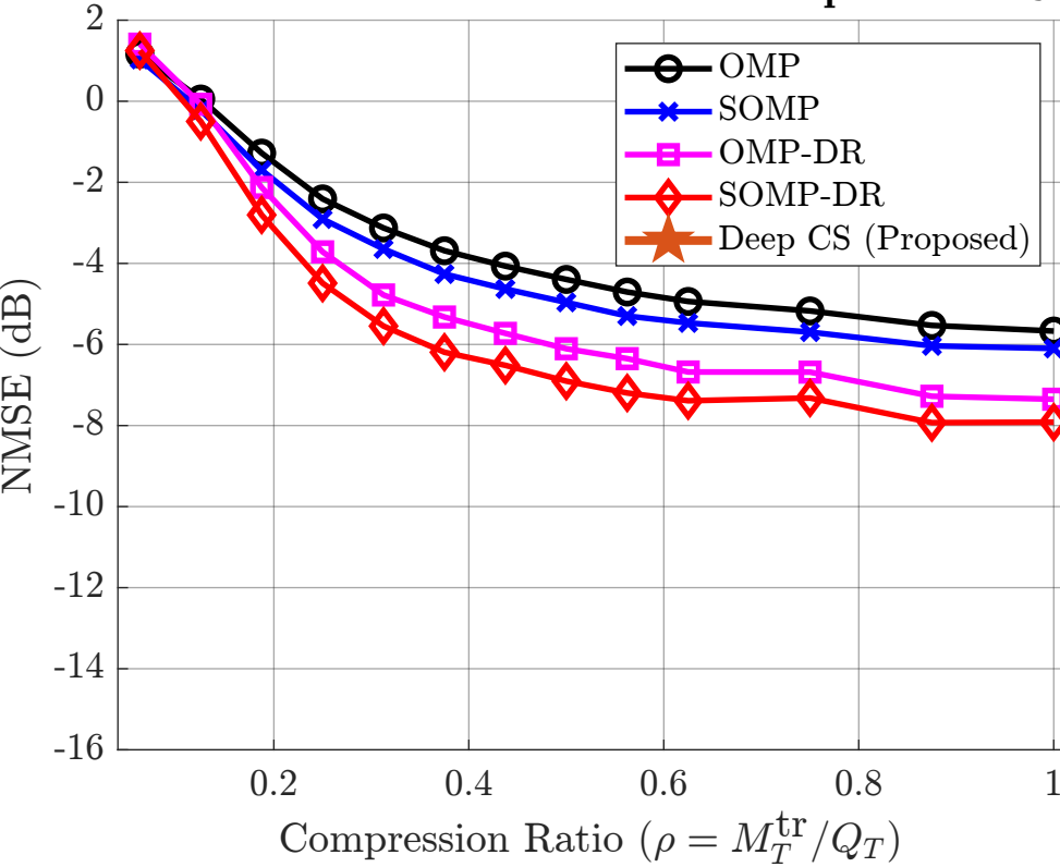
Channel Estimation NMSE vs. Compression Ratio
