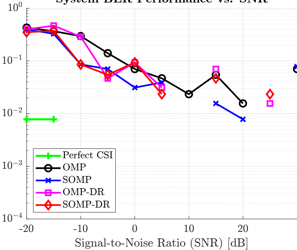
System BER Performance vs. SNR
