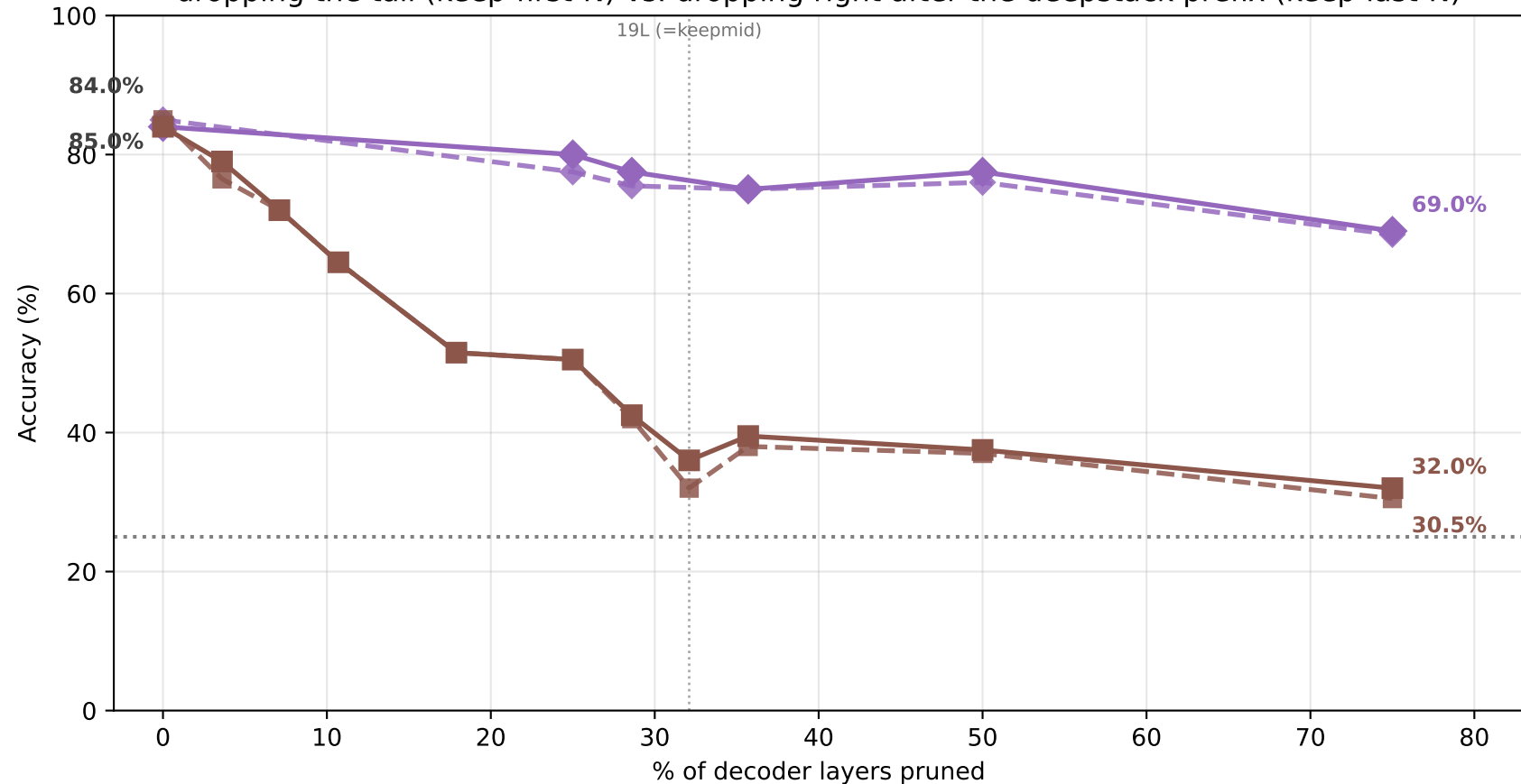
Qwen3-VL-2B depth pruning vs A-OKVQA accuracy dropping the tail (keep-first-N) vs. dropping right after the deepstack prefix (keep-last-N)
