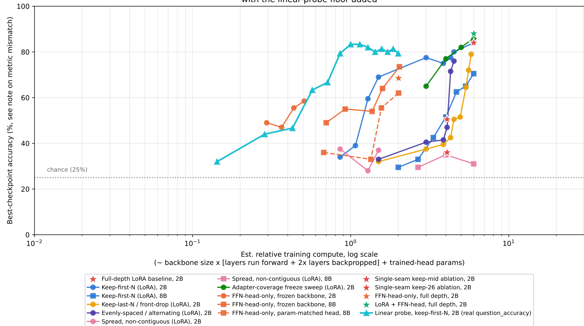
Qwen3-VL 2B & 8B on A-OKVQA: estimated training compute vs. accuracy, with the linear-probe floor added
