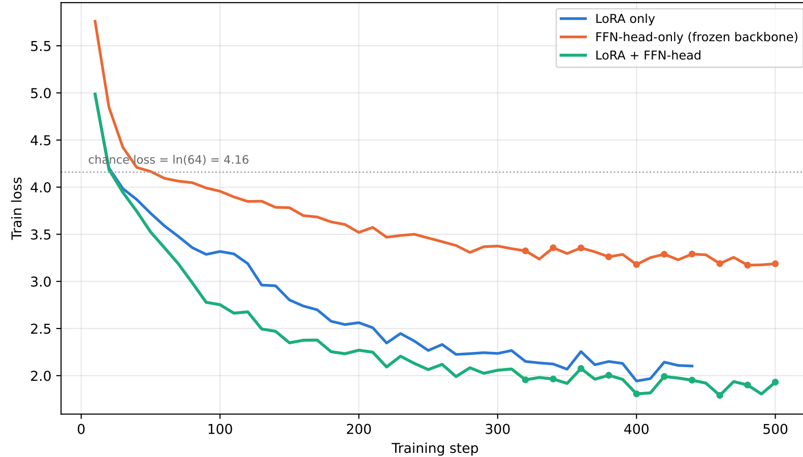
Train loss: full-depth 2B, all three methods
