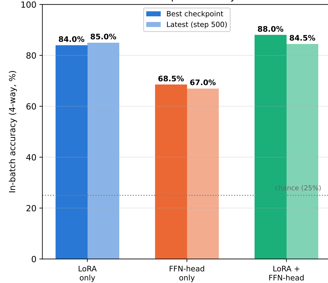
Full-depth accuracy
