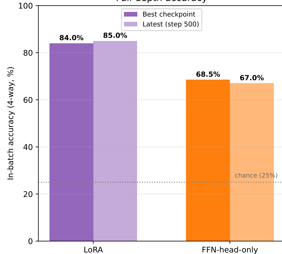
Full-depth accuracy
