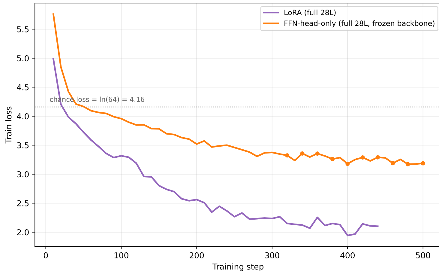
Train loss: full-depth 2B, LoRA vs. FFN-head-only
