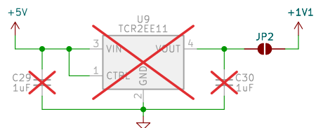
1.1V @ 200mA
