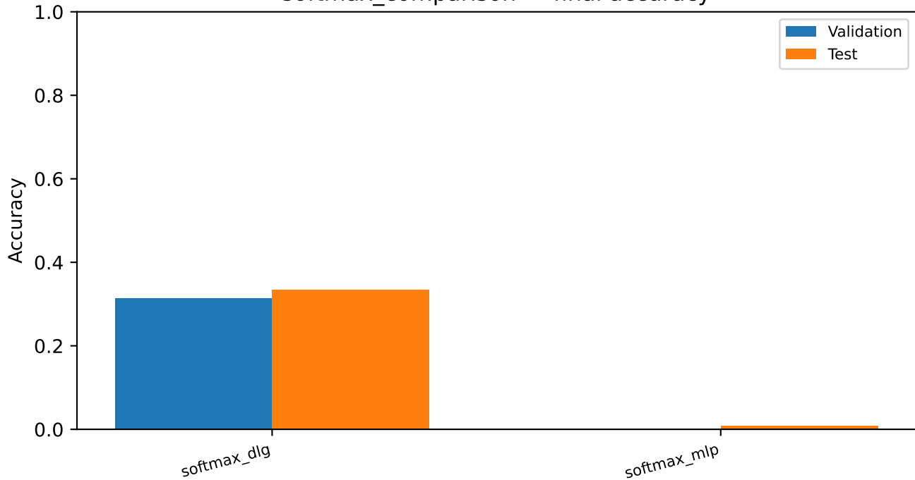
softmax_comparison — final accuracy
