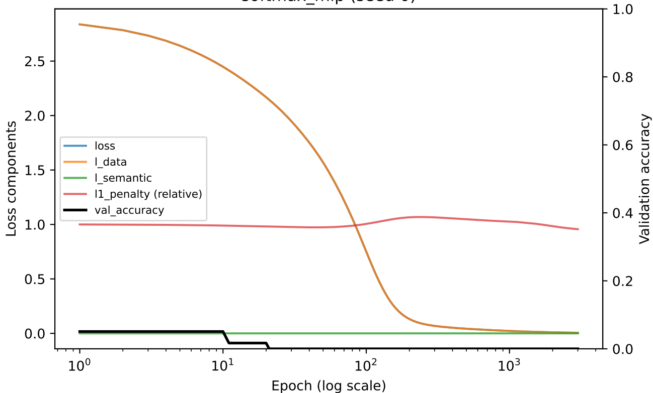
softmax_mlp (seed 0)
