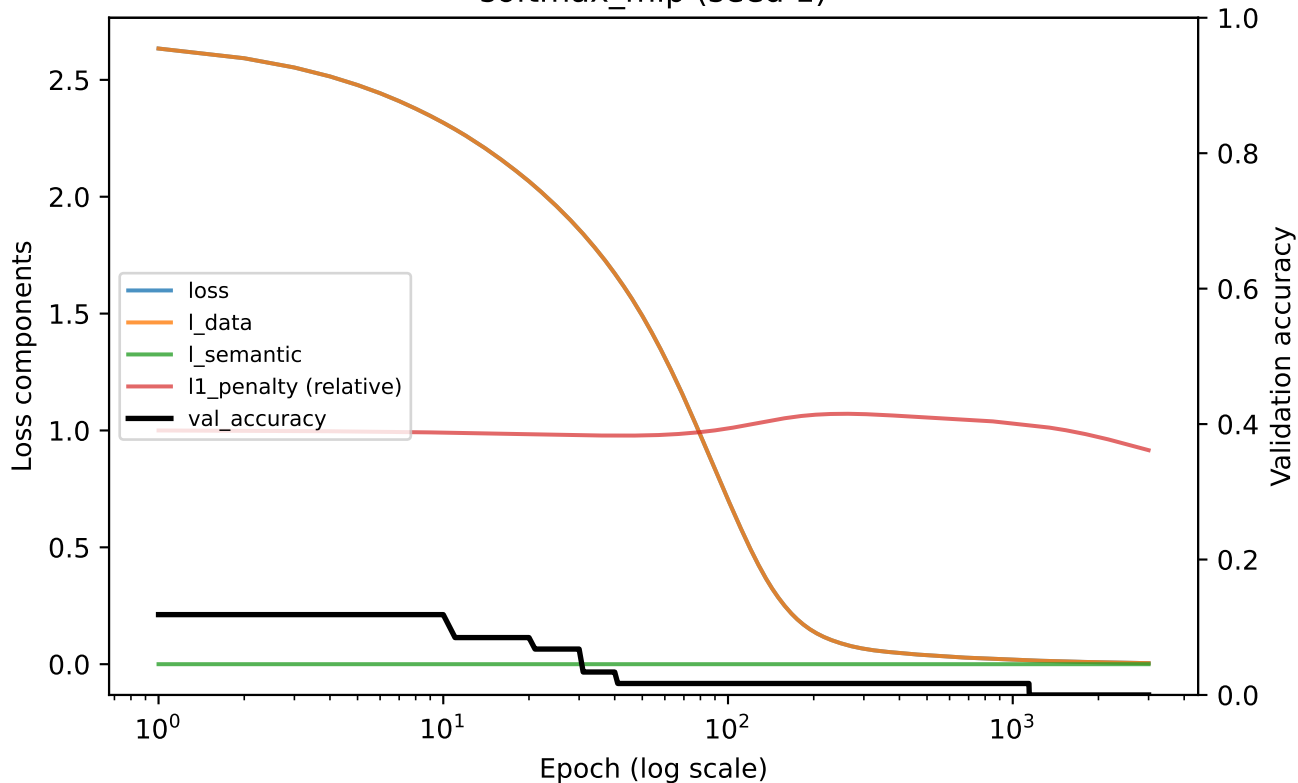
softmax_mlp (seed 1)
