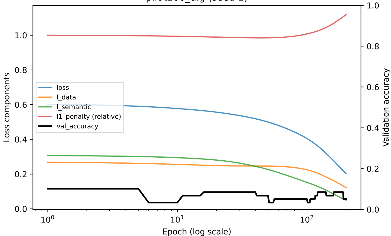
pilot200_dlg (seed 1)
