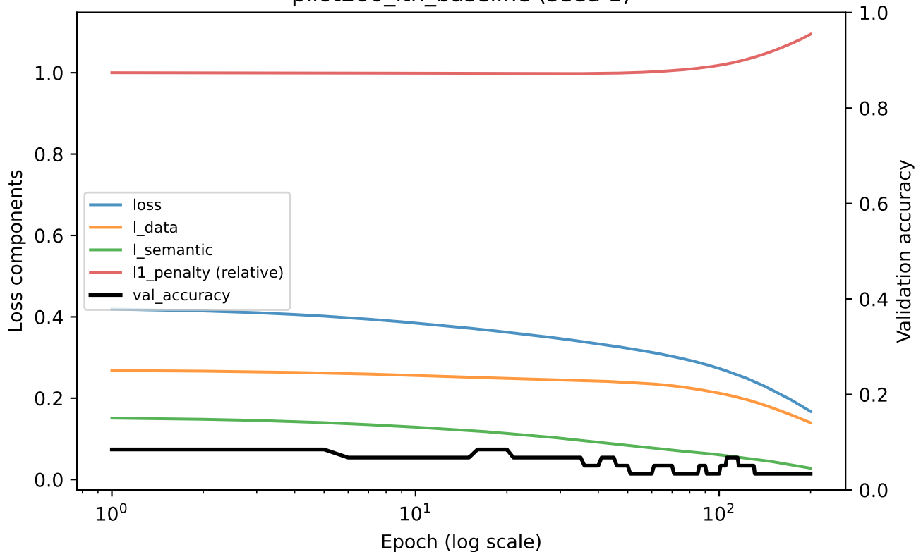
pilot200_ltn_baseline (seed 1)
