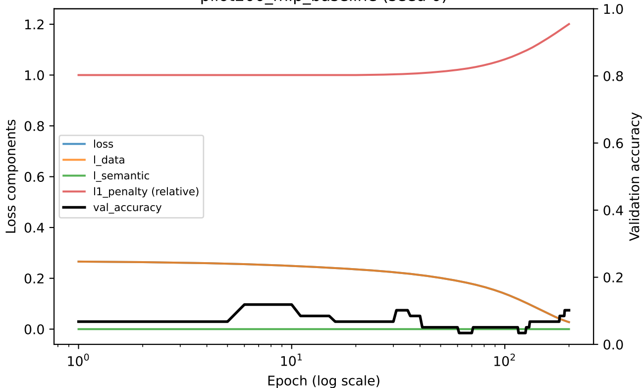
pilot200_mlp_baseline (seed 0)
