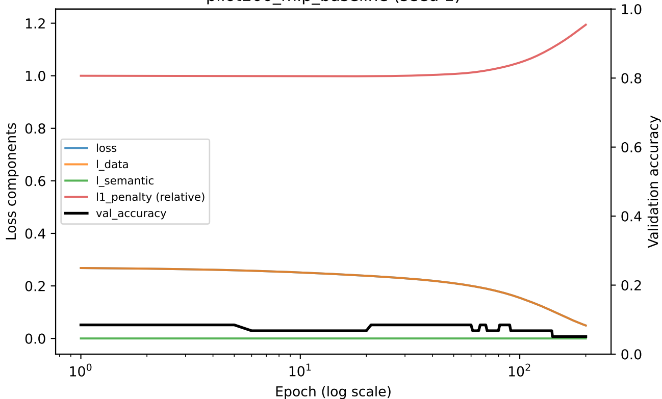
pilot200_mlp_baseline (seed 1)
