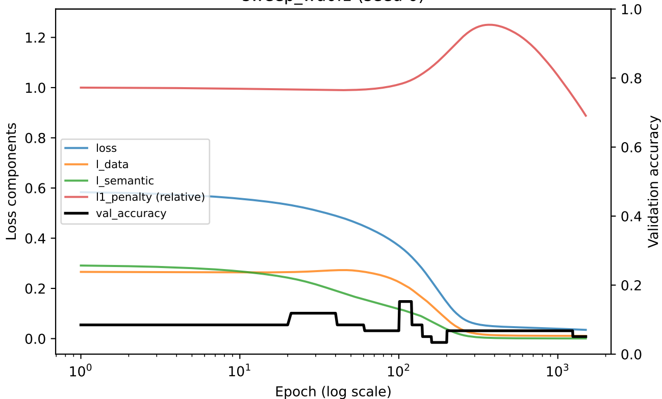
sweep_wd0.1 (seed 0)
