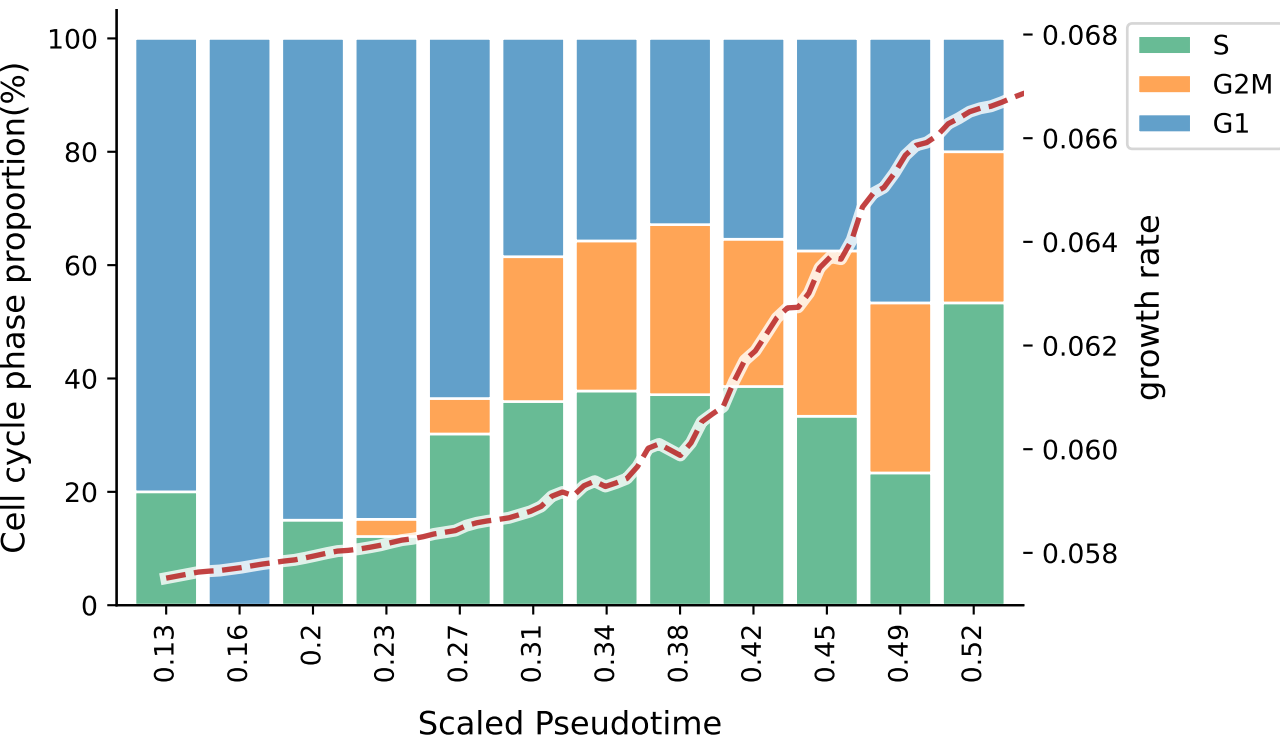
Meg Day161 growth rate & cell cycle phase
