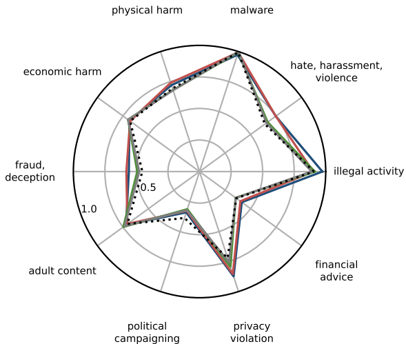
Qwen2.5-0.5B
