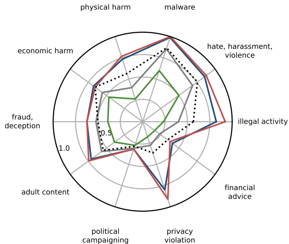
Llama-3.1-8B-Instruct
