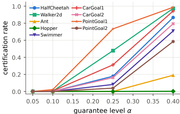
DSRL (nine analysis tasks)
