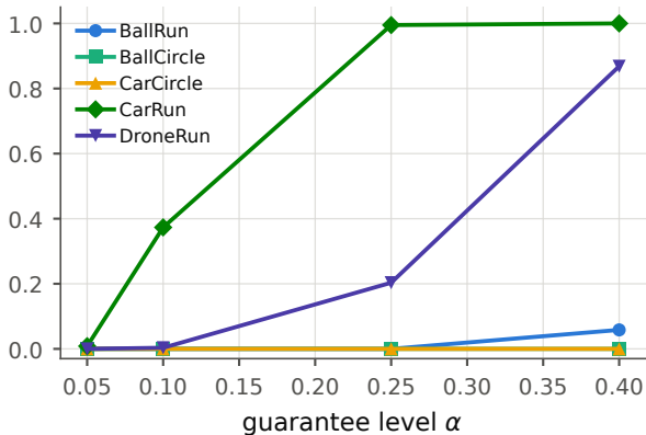
BulletSafetyGym (five tasks)
