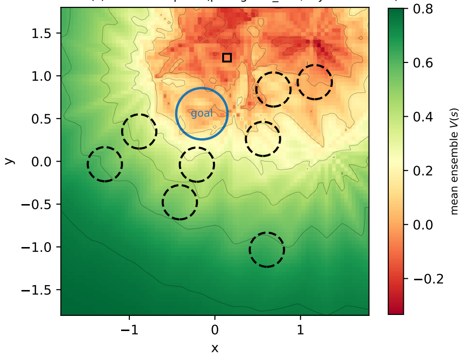
Learned V(s) over workspace (pointgoal1_dsrl, layout seed 11)
