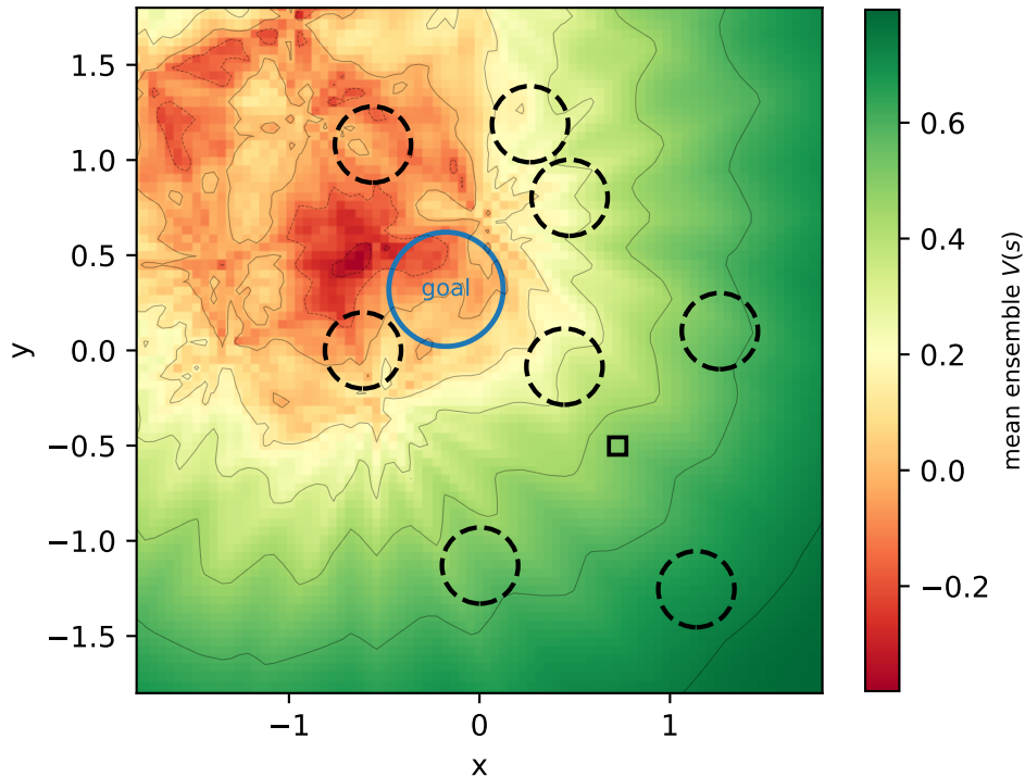
Learned V(s) over workspace (pointgoal1_dsrl, layout seed 7)
