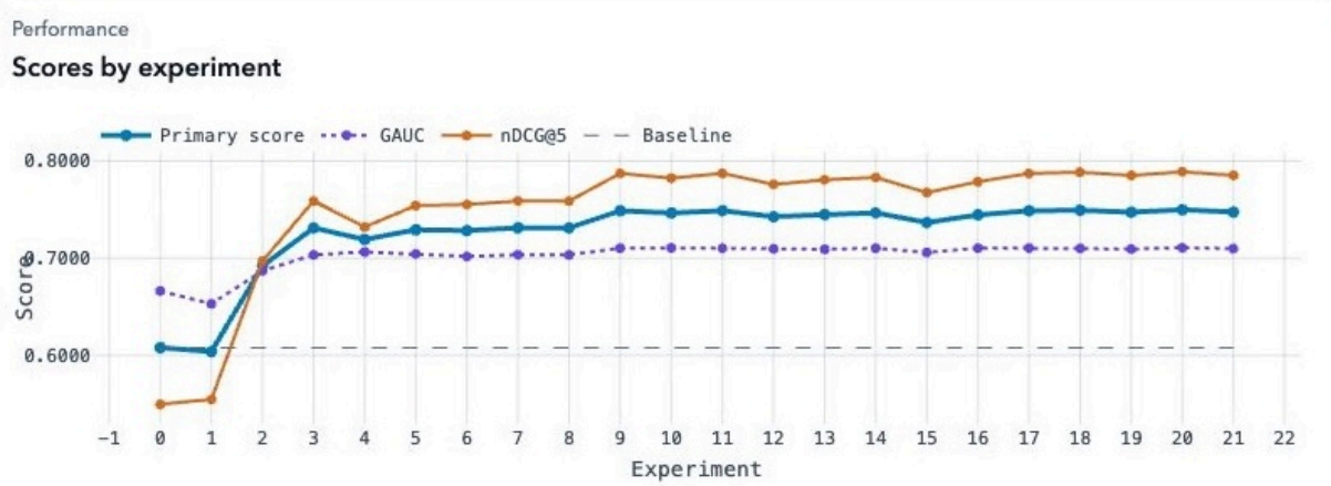
Figure 1: 1K validation trajectory. The lines show primary, GAUC, nDCG@5, and the measured reference.
