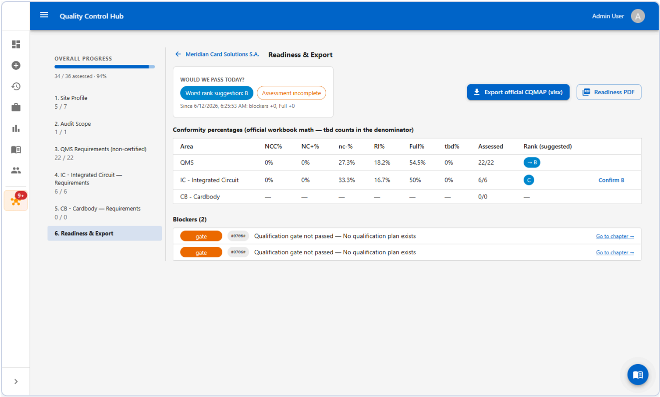
Readiness chapter with percentages, rank suggestions, and blockers
