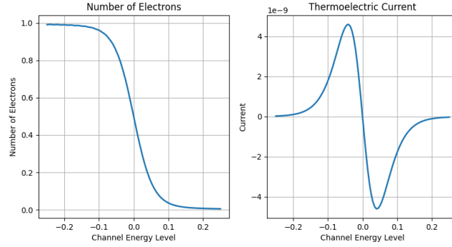
Figure 5: Thermoelectric current ( I ) and number of electrons ( N ) as functions of channel energy level ( \mathcal{E} ).
