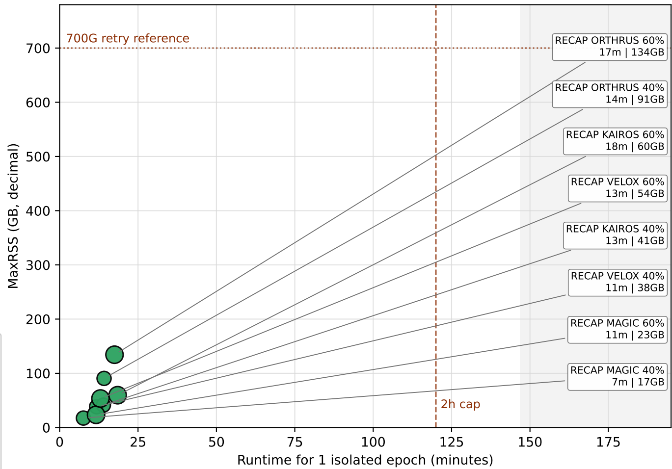
RECAP
