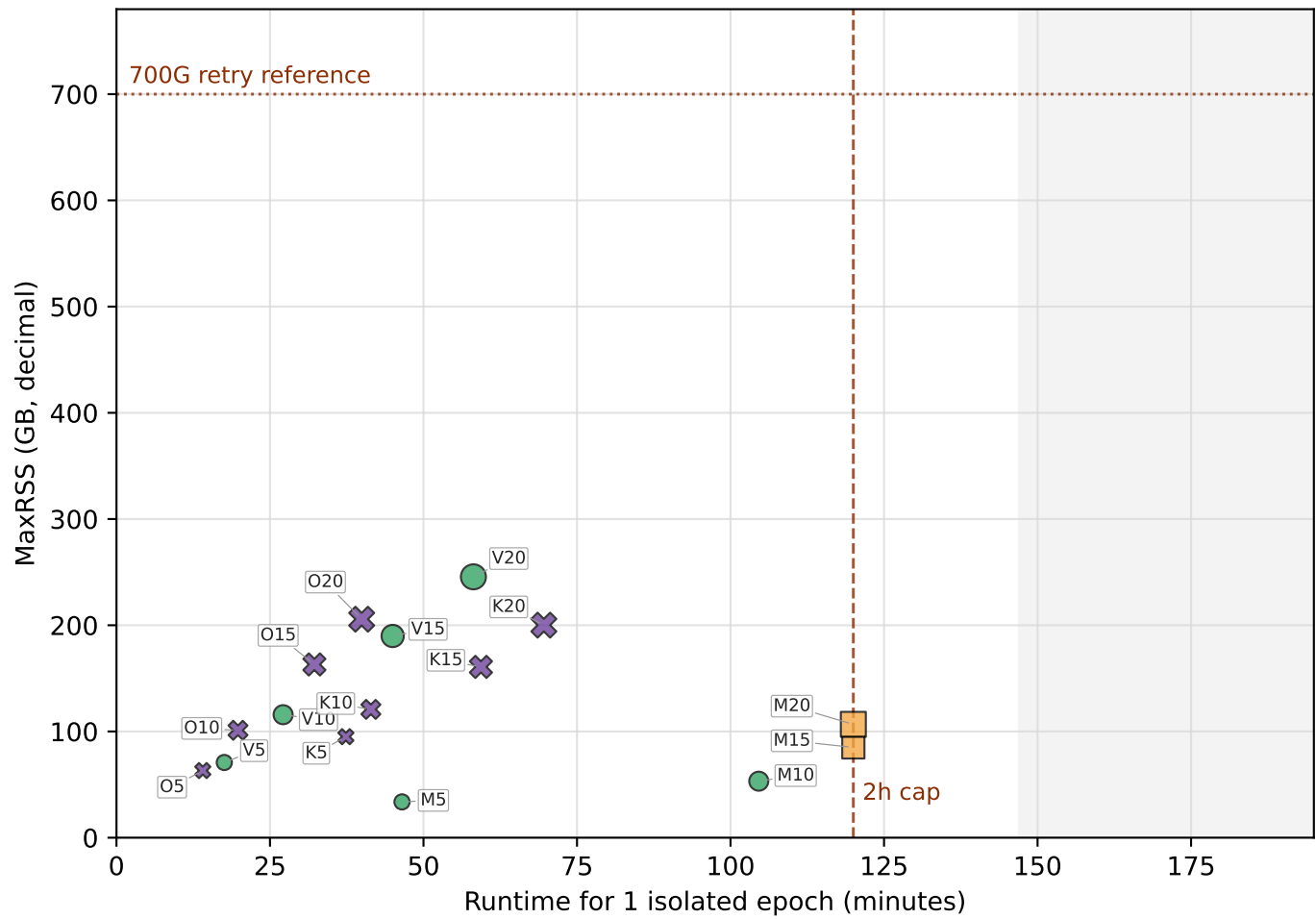
CamFlow
