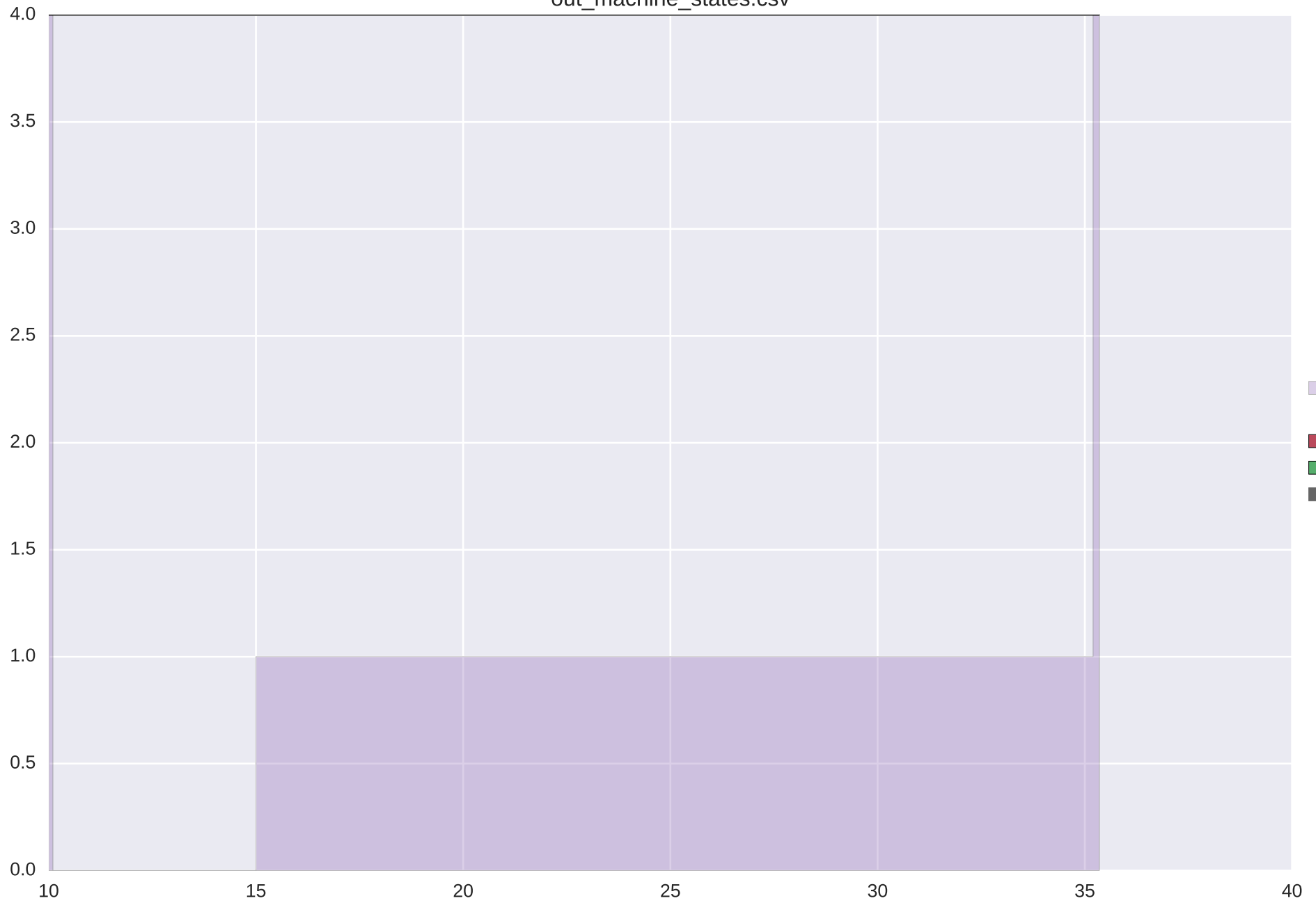
out_machine_states.csv
