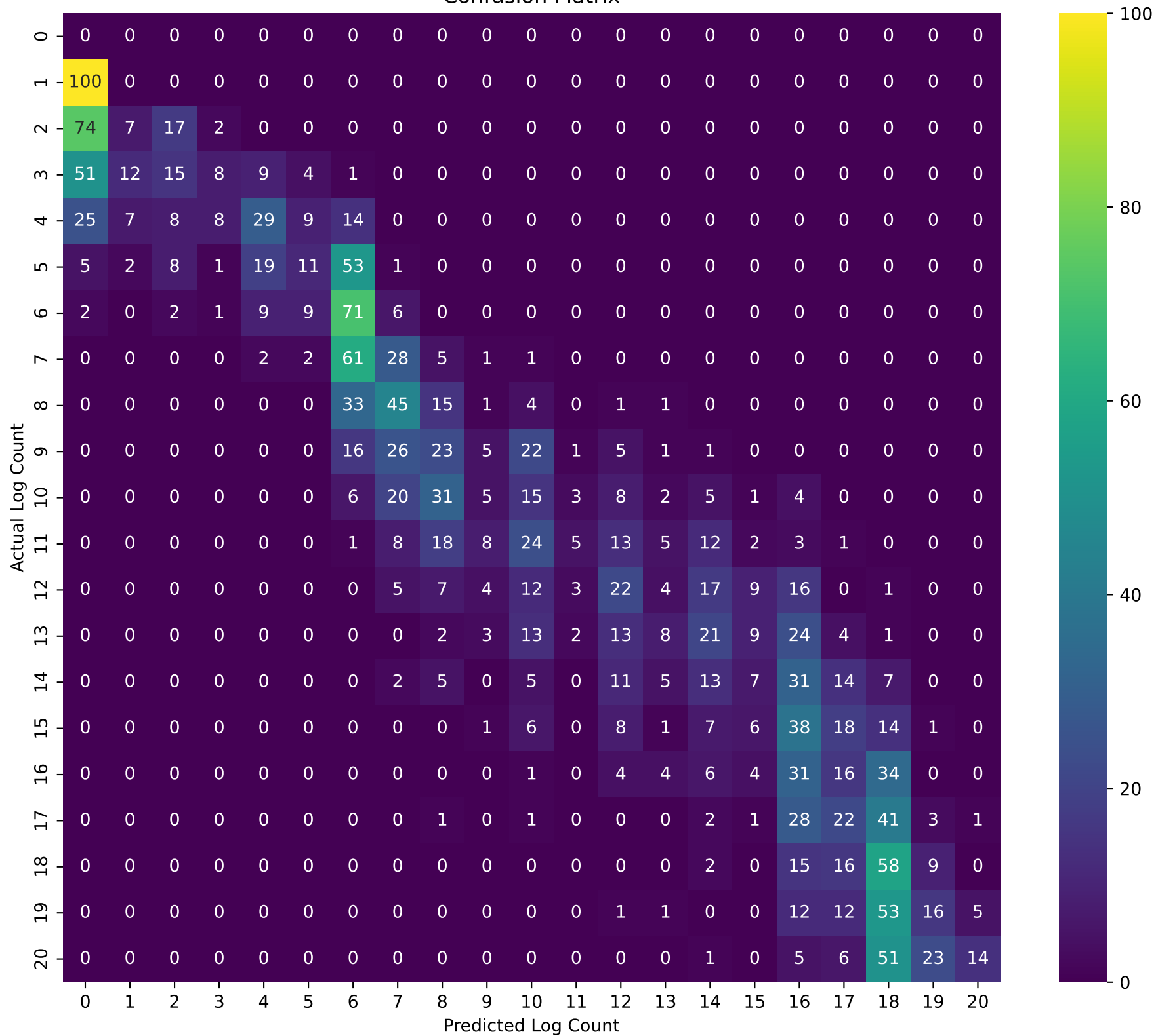
Confusion Matrix
