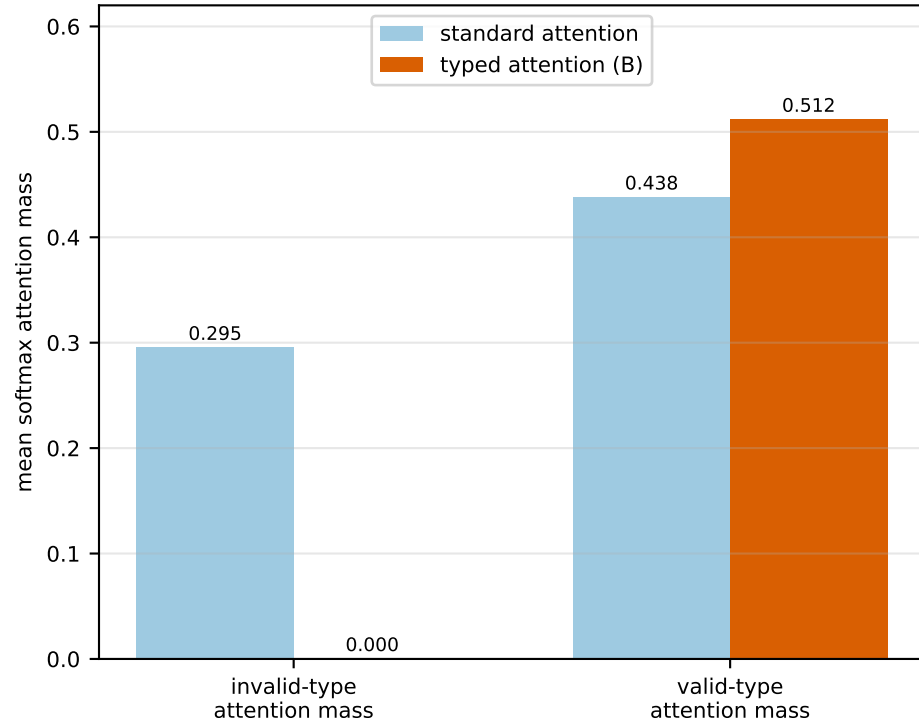
(b) Measured effect (seed 42, 300 epochs) typed attention drives invalid mass to zero
