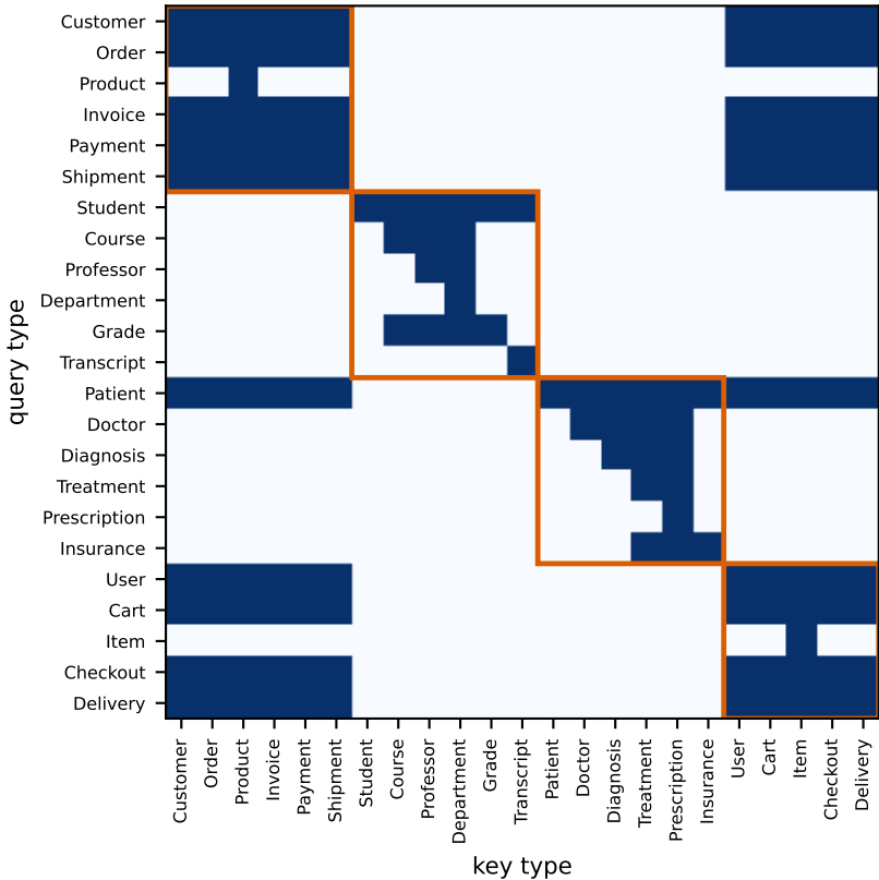
(a) Olog reachability mask enforced by (B) shaded = attention permitted; boxes = domain blocks
