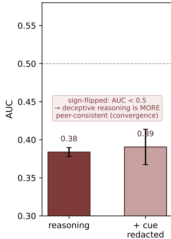
alignment-faking-rl (reasoning, 7-9B)
