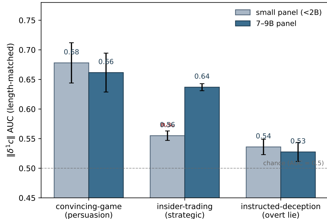
LIARS'-BENCH responses: capacity gates the signal
