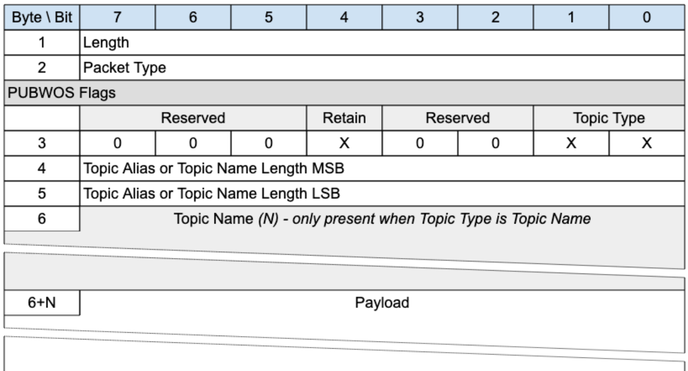
Figure 11: PUBWOS Packet
