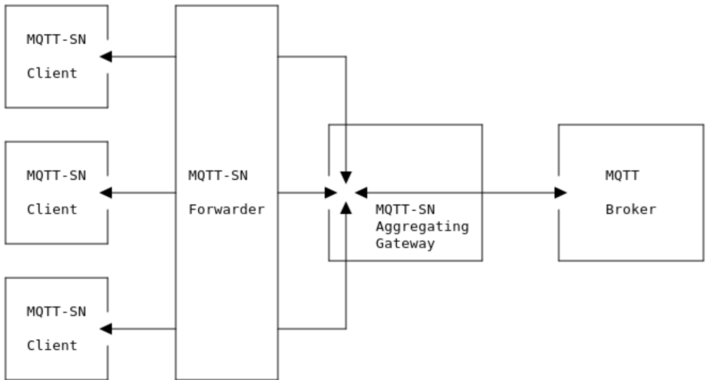
Figure 40: Forwarder with Aggregating Gateway
