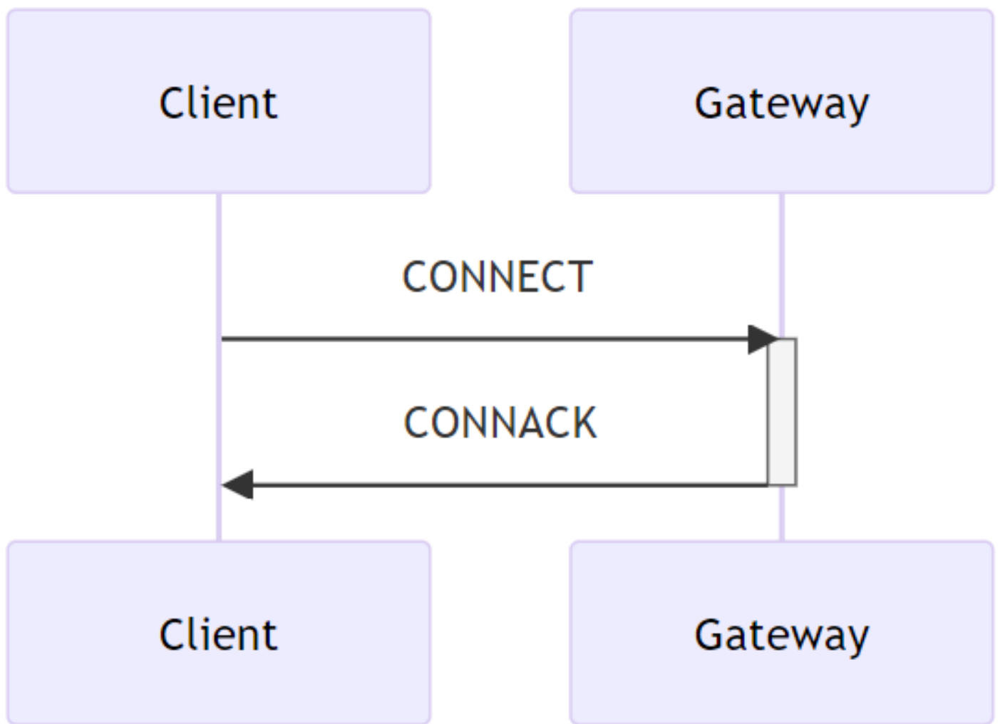
Figure 34: Connect Procedure (without Auth flag set, or no further authentication data required)
