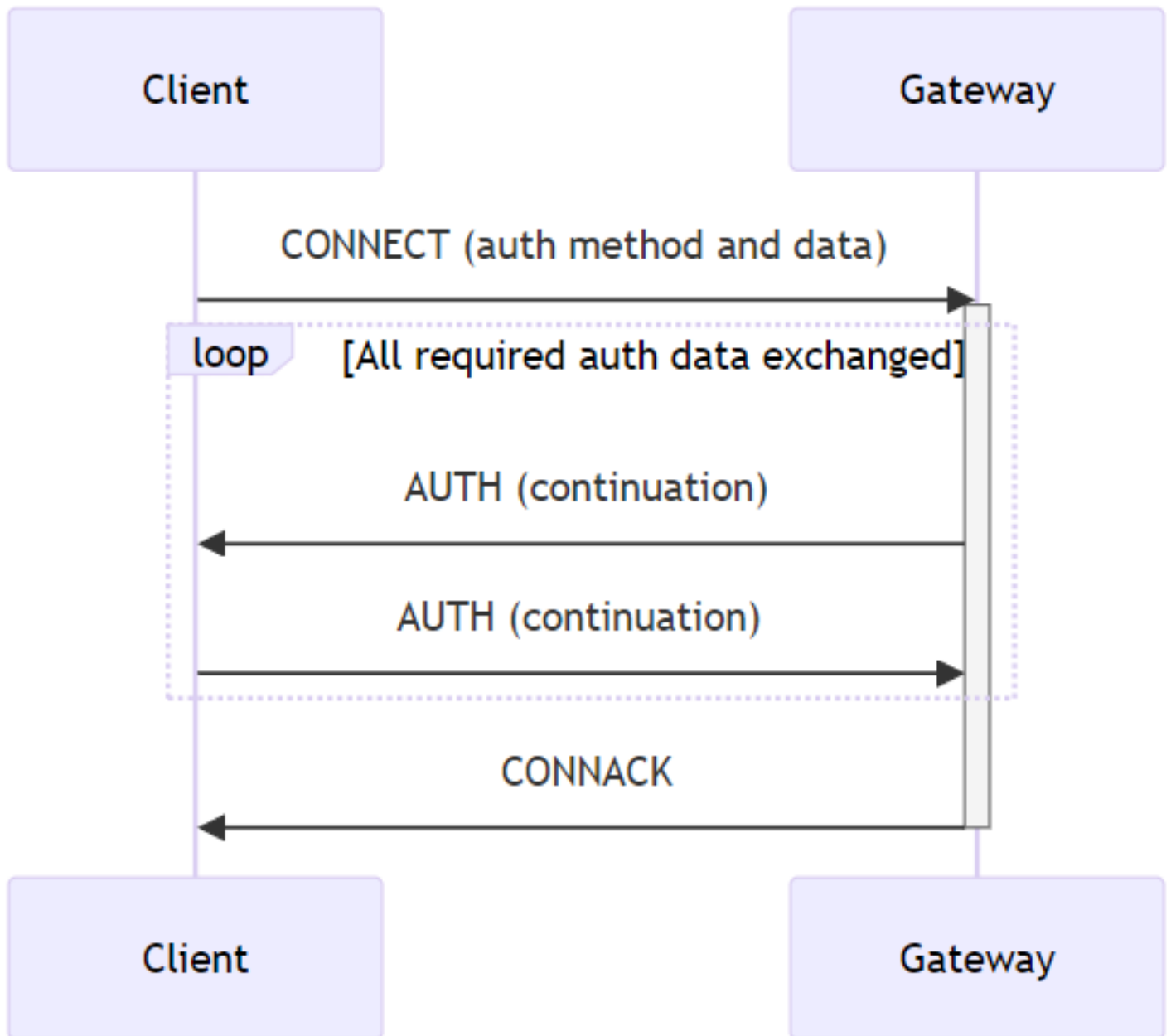
Figure 35: Connect Procedure (with Auth flag set and further authentication data required)
