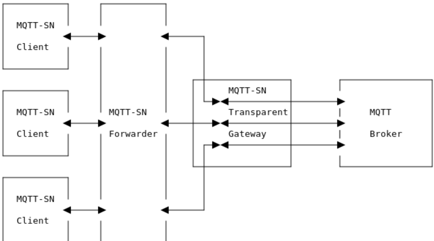
Figure 39: Forwarder with Transparent Gateway
