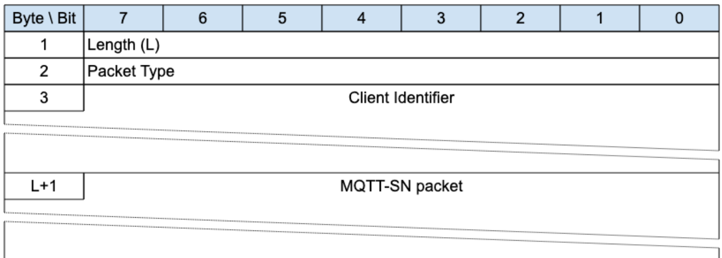
Figure 29: Format of a Connection Encapsulated MQTT-SN Packet
