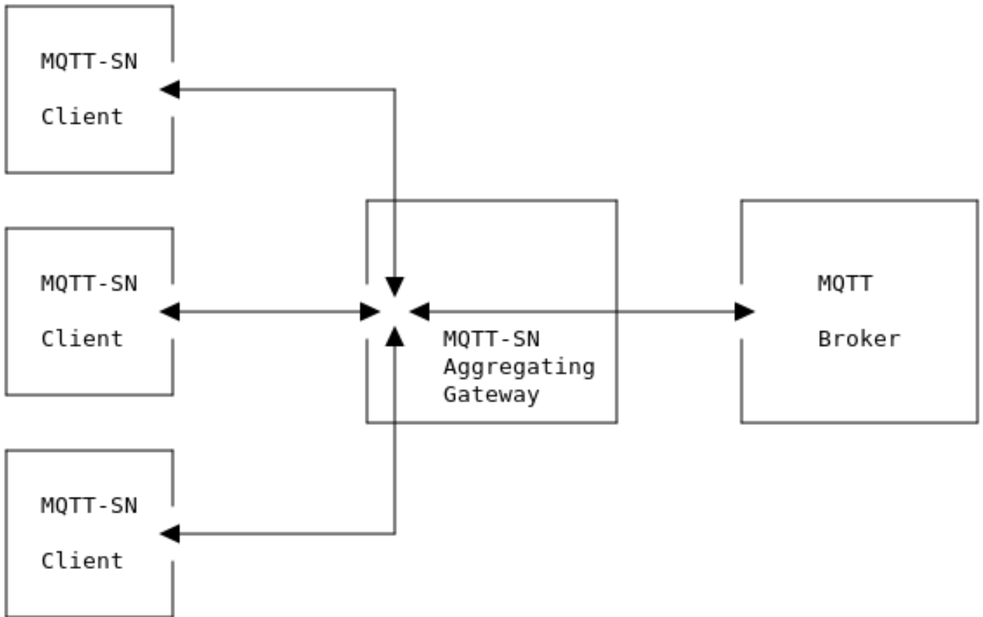
Figure 38: Aggregating Gateway
