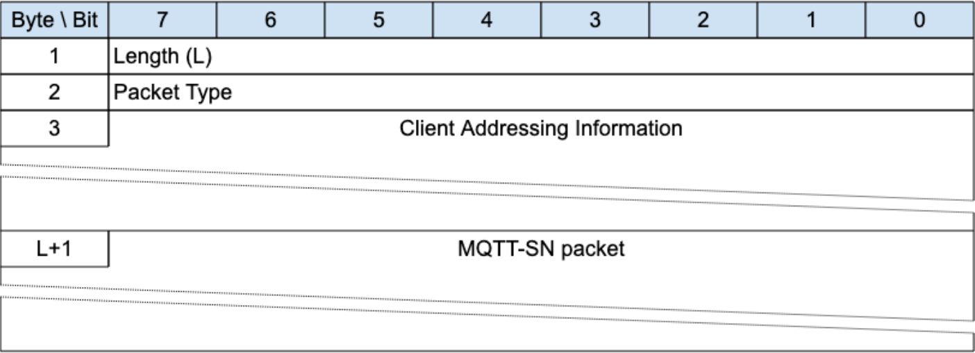
Figure 30: Format of an Forwarder Encapsulated MQTT-SN Packet
