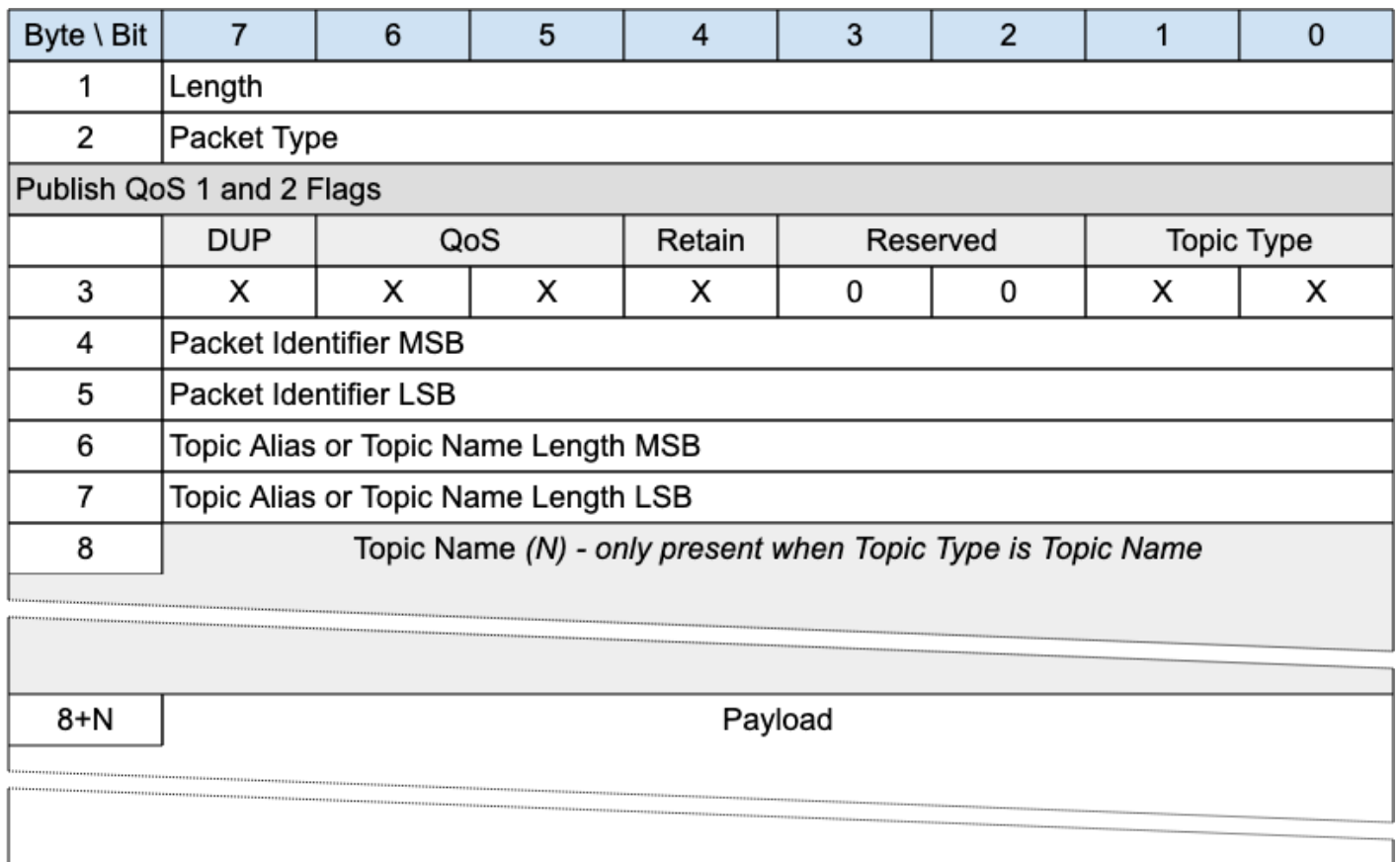
Figure 13: PUBLISH Packet for QoS 1 and 2
