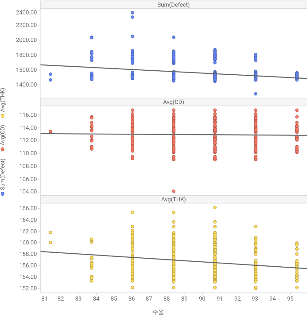
Sum(Defect), Avg(CD), Avg(THK) vs. 수율
