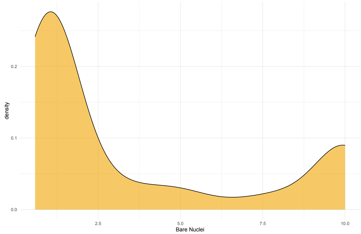
Density: Regression with Perturbation Maintains natural variance/noise
