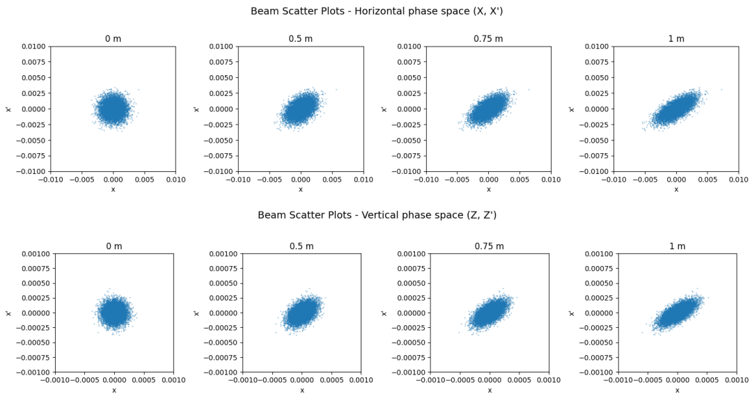
Figure 18: Evolution of the phase space. Top: in X (horizontal), bottom: in Z (vertical).
