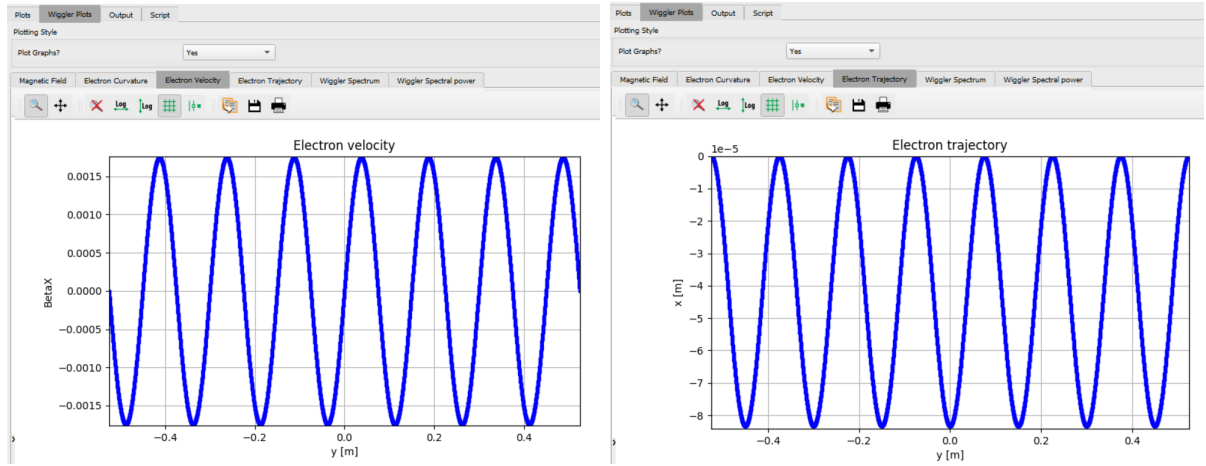
Figure 9: Electron transversal velocity (left) trajectory (right). Note that the velocities are centred, but not the trajectories. By default, the electron enters the wiggler at x = 0 .
