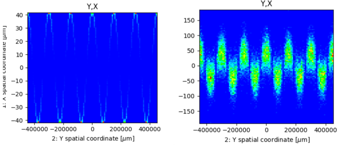
Figure 13: Top view of the emission x(y) for the wiggler placed in a zero emittance ring (left), or in a ring with emittance (right)
