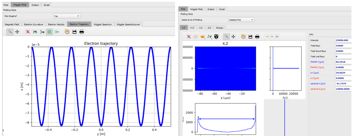
Figure 10: Electron trajectory (left), and source emission. Note that the non-centered trajectory imply that the photon source is not centered at zero. This is “corected” in next figure.
