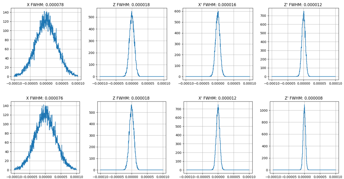
Figure 15: Like figure ?? but with electron energy spread considered. Observe the increase of the divergences for the high harmonics.
