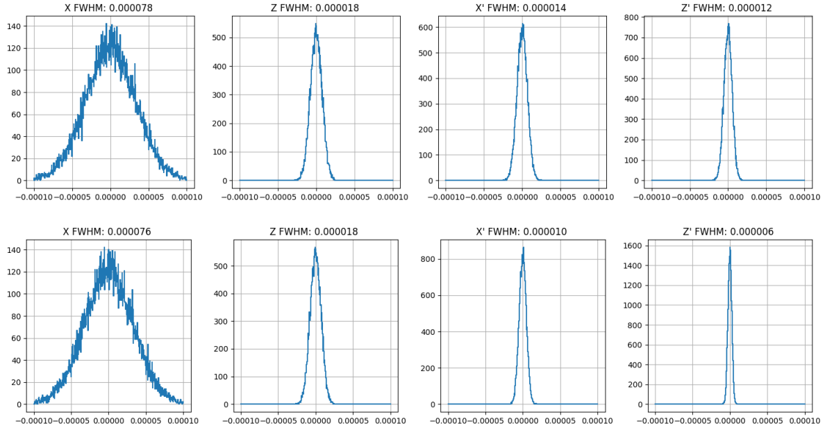
Figure 14: Intensity distribution for real space (X,Z) and divergence space (X', Z') for an undulator (Gaussian approximation) at E_1=15 keV (top) and E_9=135 keV (bottom). No electron energy spread considered.
