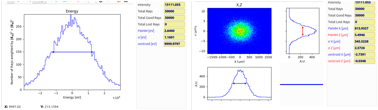
Figure 32: Bandwidth and image at best focus for off-Rowland ( R=50 m) configuration.
