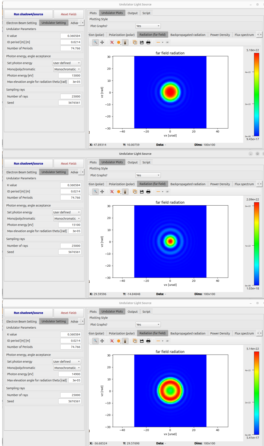
Figure 16: In the “Undulator Light Source” widget, manual set of the far field radiation at resonance E_1 (top), at E_1+100 eV (center), and E_1-100 eV (bottom).
