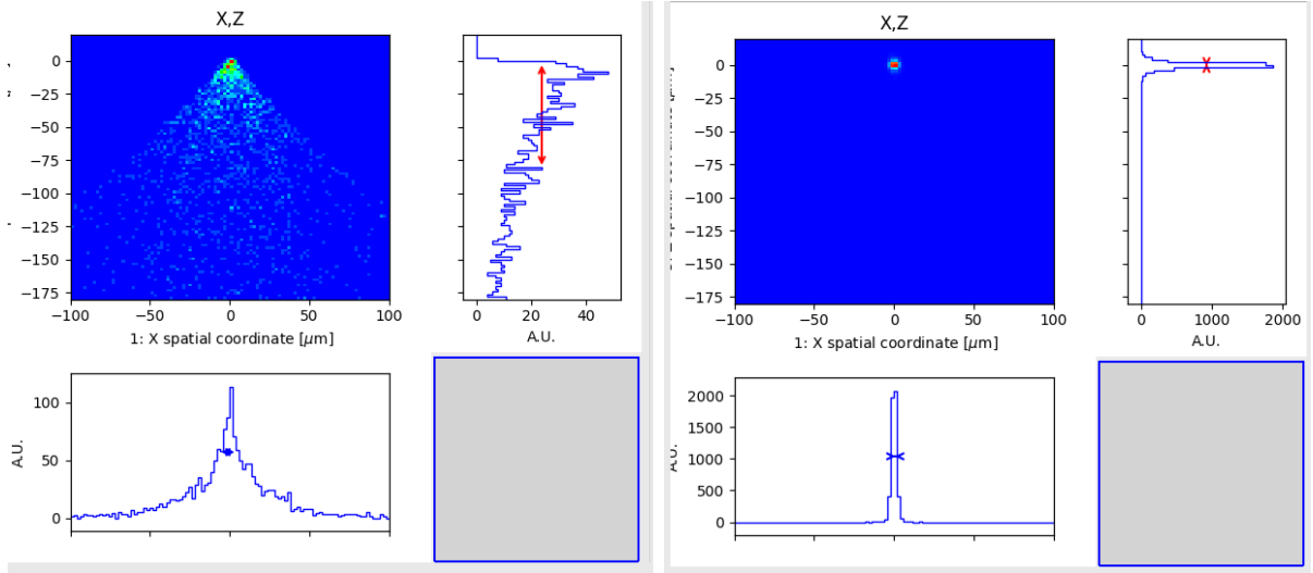
Figure 21: Mirror imaging with magnification M=1/30 : Toroidal (left) and Ellipsoidal (right).
