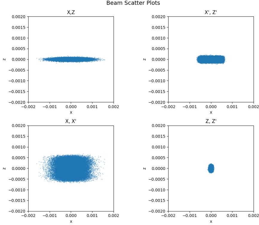
Figure 6: Rays in real space (X,Z) , divergence space (X',Z') , phase space (X,X') along column 1, and phase space (Z,Z') along column 2,
