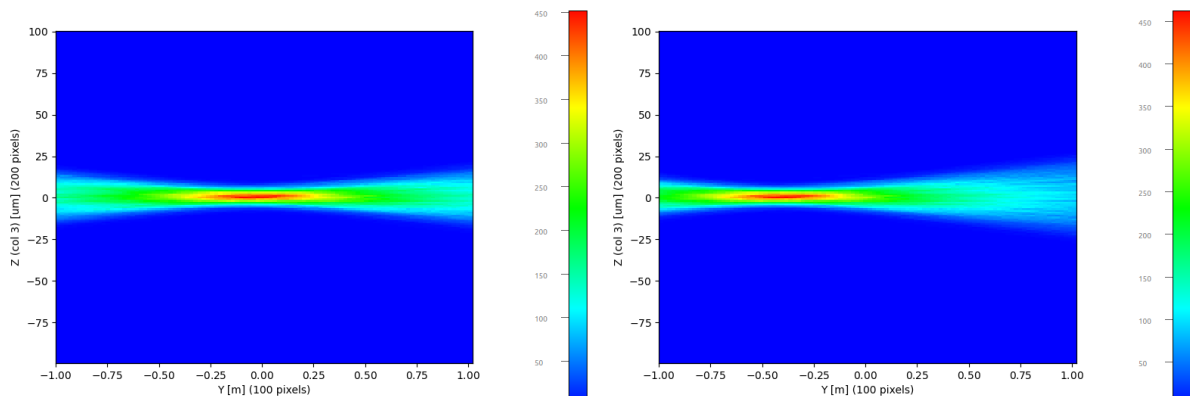
Figure 34: Caustic (vertical beam size vs propagation direction) at 35.7 keV (left) that is the energy used to tune the transfocator, and also at 35.2 keV (right) where it can be observed a shift of the focal position at about 0.4 m upstream from the image plane. This illustrates the chromatic aberrations of the lenses.
