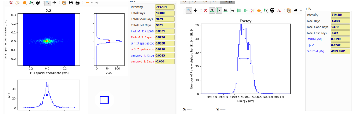
Figure 35: Ray tracing results in terms of intensity distribution in the (X,Z) plane at the image position (left), and energy resolution (right).
