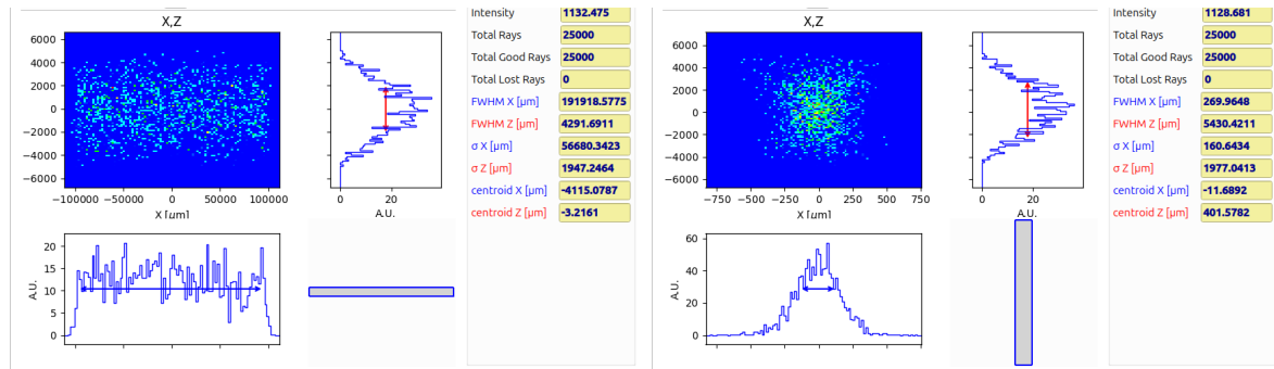
Figure 27: Image at focal plane by the flat-flat system (left) and the flat-sagittal system (right)
