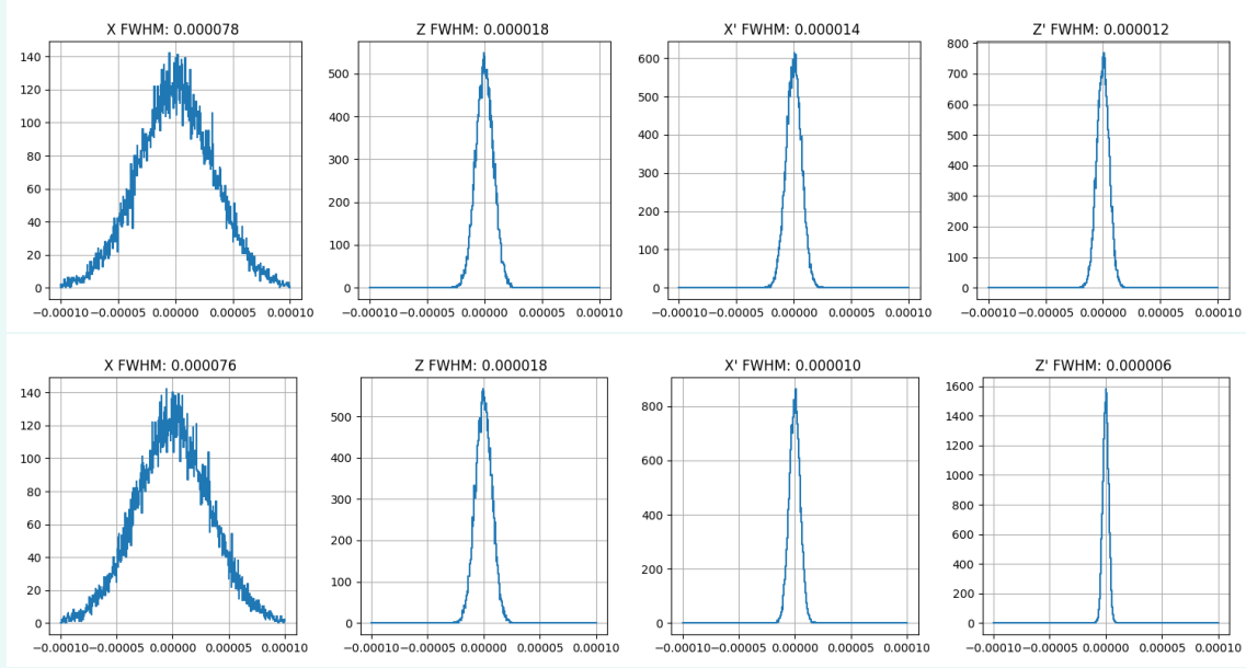
Figure 14: Intensity distribution for real space (X,Z) and divergence space (X', Z') for an undulator (Gaussian approximation) at E_1=15 keV (top) and E_9=135 keV (bottom). No electron energy spread considered.
