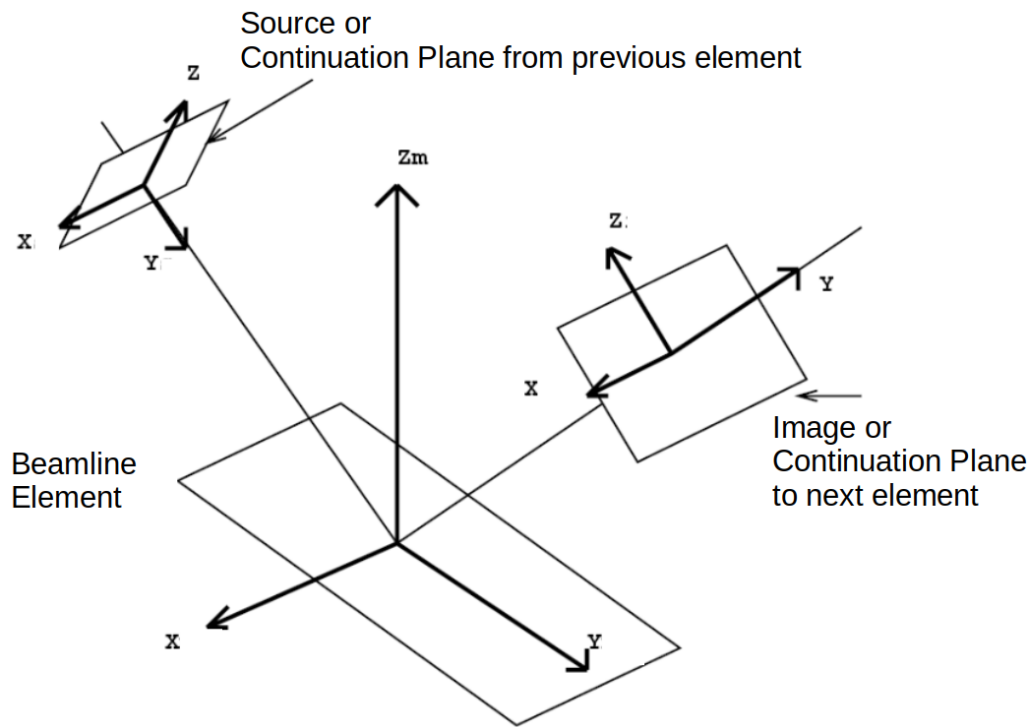
Figure 1: SHADOW4 reference frame definitions: Source, beamline element, and image coordinates.
