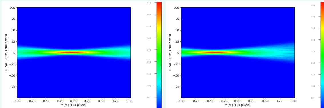
Figure 34: Caustic (vertical beam size vs propagation direction) at 35.7 keV (left) that is the energy used to tune the translocator, and also at 35.2 keV (right) where it can be observed a shift of the focal position at about 0.4 m upstream from the image plane. This illustrates the chromatic aberrations of the lenses.
