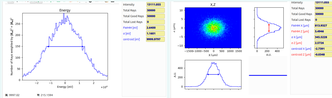
Figure 32: Bandwidth and image at best focus for off-Rowland ( R=50 m) configuration.
