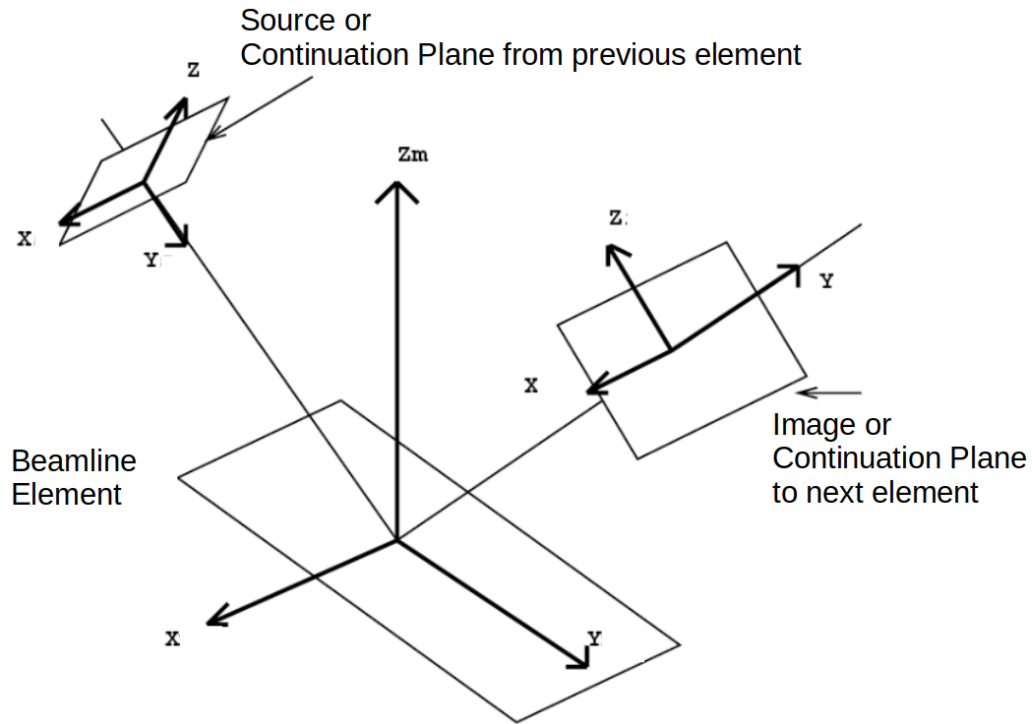
Figure 3: SHADOW4 reference frame definitions: Source, beamline element, and image coordinates.
