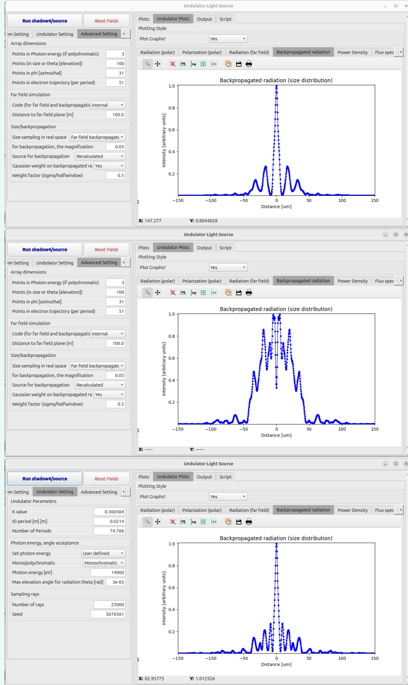
Figure 17: In the “Undulator Light Source” widget, manual set of the backpropagating the far field radiation at resonance E_1 (top), at E_1+100 eV (center), and E_1-100 eV (bottom).
