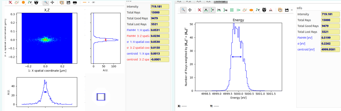
Figure 35: Ray tracing results in terms of intensity distribution in the (X,Z) plane at the image position (left), and energy resolution (right).
