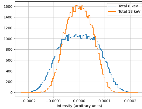
Figure 8: Histograms of the total intensity vs Z' for emission at 8 and 18 keV.
