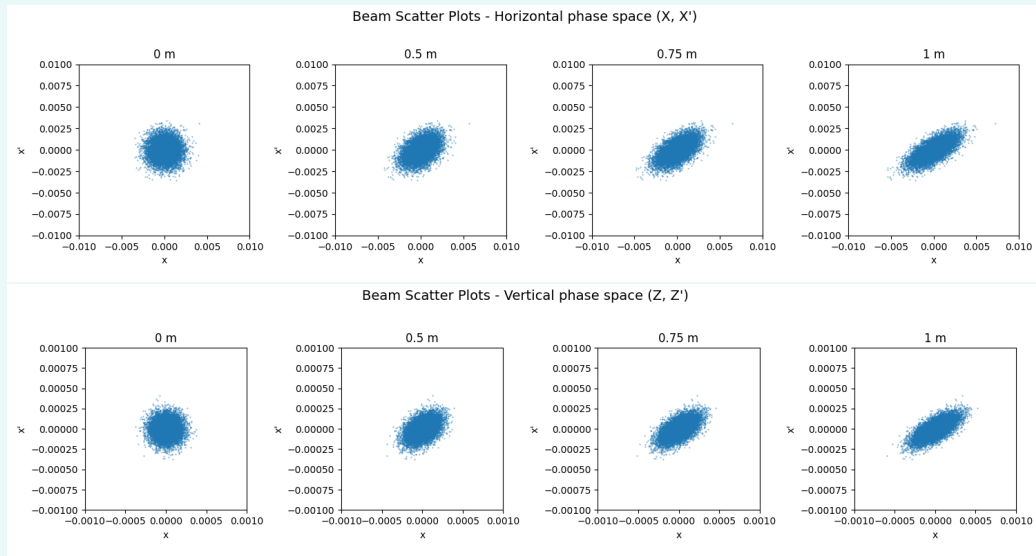
Figure 18: Evolution of the phase space. Top: in X (horizontal), bottom: in Z (vertical).
