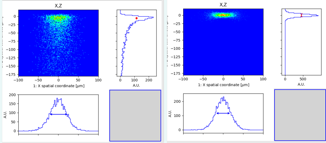
Figure 20: Mirror imaging with magnification M=1/3 : Toroidal (left) and Ellipsoidal (right).
