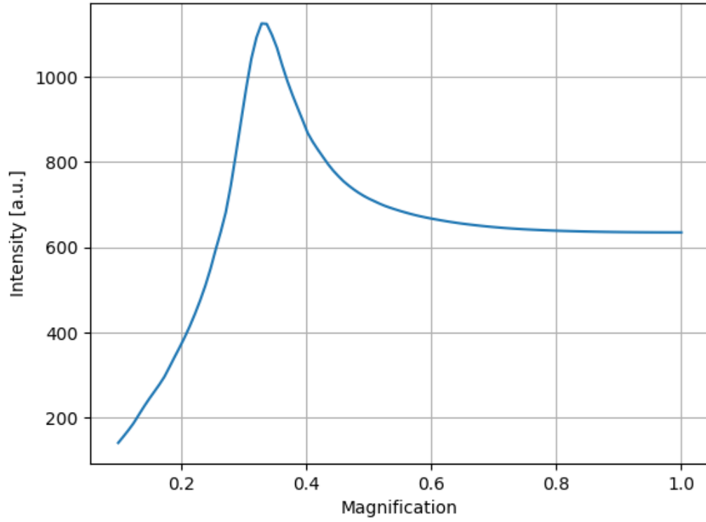
Figure 28: Intensity (in arbitrary units) versus magnification factor M for a point and monochromatic ( E=20 keV) source placed at 30 m from the sagittally bent crystals. The beam divergences is 5 mrad. We clearly observe the maximum of the transmission at M=0.33 , as predicted by the theory.
