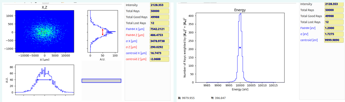
Figure 29: No bump: H: 7.5 mm, V: 0.49 m, \Delta E=1.2 eV
