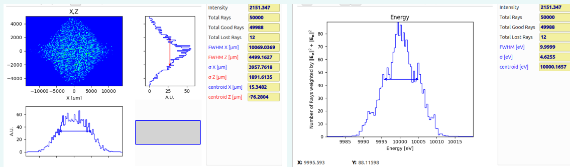
Figure 30: With bump: H: 10 mm, V: 4.5 mm, \Delta E=10 eV
