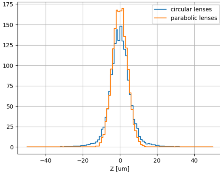
Figure 33: Intensity distribution in vertical direction at the image (focal) plane for a CRL with circular lenses and parabolic lenses.
