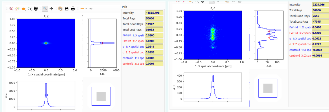
Figure 23: Intensity distribution at the focal plane produced by the KB. Left: ideal surfaces without slope errors. Right: using slope errors from measured data (DABAM library) ( 0.91 \mu\text{rad} r.m.s. for VFM and 0.51 for HFM).
