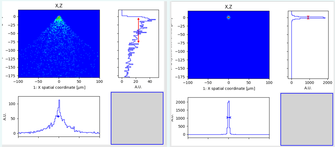
Figure 21: Mirror imaging with magnification M=1/30 : Toroidal (left) and Ellipsoidal (right).
