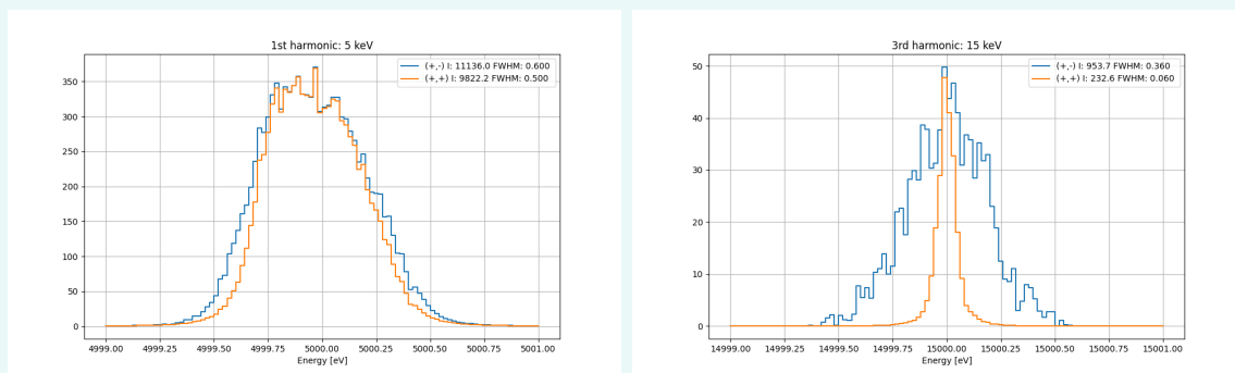
Figure 26: Intensity vs photon energy plots for the two configurations (+,-) and (+,+). Left: 1 st harmonic around 5 keV. Right: 3 rd harmonic around 15 keV.
