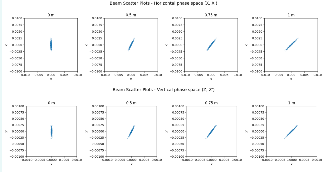
Figure 19: Evolution of the phase space. Effect of a slit in the first screen. Top: in X (horizontal), bottom: in Z (vertical).
