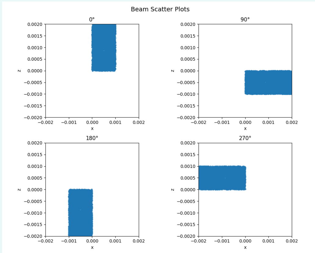
Figure 5: Effect of an empty element in the beam for different \alpha . Note that the beam is unchanged, but the axes are rotated and displayed in the same configuration, therefore there is an apparent rotation of the beam.
