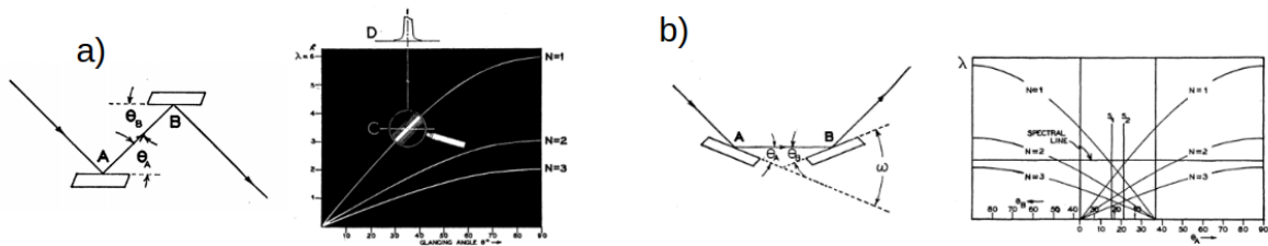
Figure 25: Du Mond diagrams for a) (+,-) configuration, and b) (+,+) configuration. J. W. M., DuMond, Phys. Rev. 52, 1937, 872-883.
