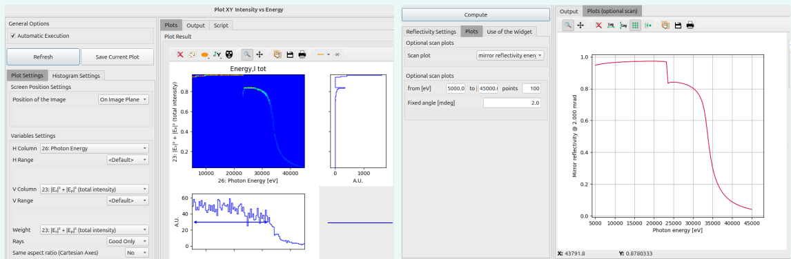
Figure 22: I(E) plot from rays (left) or from PreRefl preprocessor (right).
