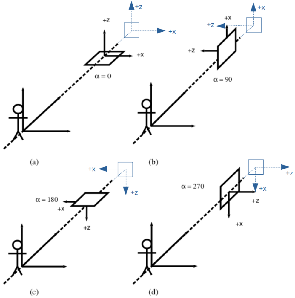
Figure 4: Effect of the beamline element orientation angle \alpha for the four most common values: 0, 90, 180 and 270 degrees. The effect of the angle \alpha is carried out to the image plane, thus defining the position of the axes (in blue).
