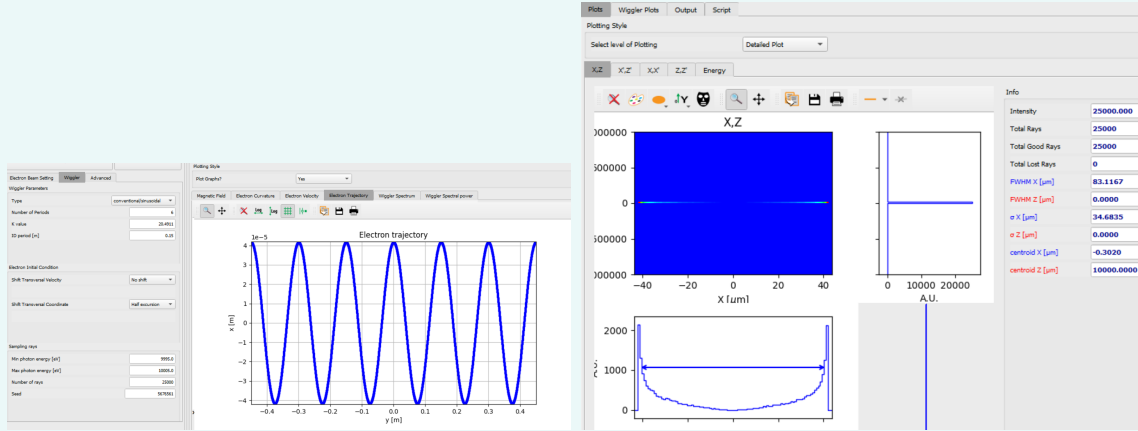
Figure 11: Electron trajectory corrected to place the center at “half-excursion” (left), and source emission. Note that the centered trajectory imply that the photon source is now centered at zero.
