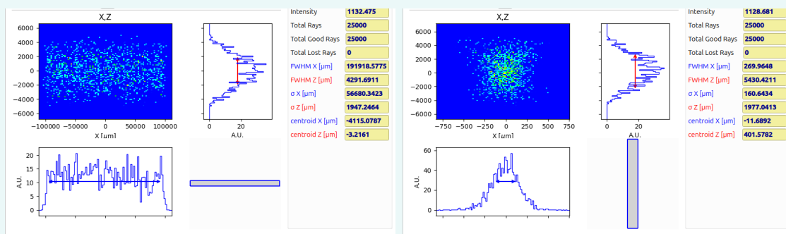
Figure 27: Image at focal plane by the flat-flat system (left) and the flat-sagittal system (right)
