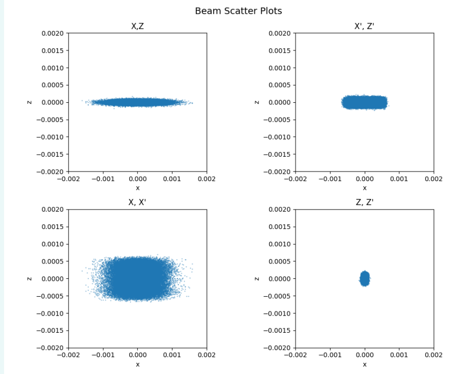
Figure 6: Rays in real space (X,Z) , divergence space (X',Z') , phase space (X,X') along column 1, and phase space (Z,Z') along column 2.
