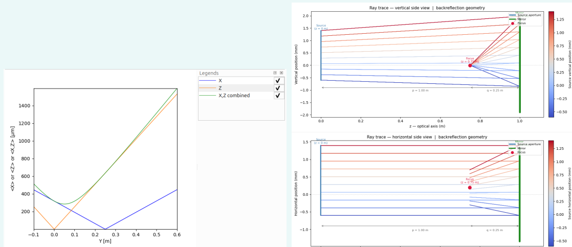
Figure 2: Left: beam evolution (from FocNew). In vertical (Z), the best focus is at zero (at the image plane). In horizontal (X) the best focus is at 0.25 m downstream from the image plane, as a result of astigmatism provoked by the non-normal incidence with spherical reflectors. Right: diagram of the path of the rays.
