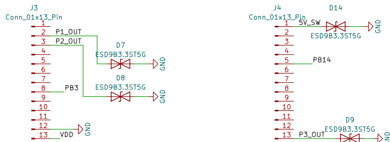
Output Headers to Dragino/LoRaWAN
